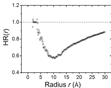
FIGURE 4 HR(r) (circles) as a function of the radial distance r from the Mg^{2+} ion. The dotted reference line represents the fully hydrated Mg^{2+} ion in the bulk solution.
