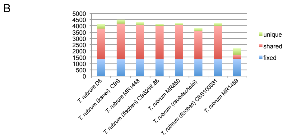
Figure S3. Phylogenetic relationship and sharing of variant sites of sequenced T. rubrum isolates. A. Phylogenetic relationship of T. rubrum isolates inferred using RAxML (Methods). B. Classification of SNP sites based on conservation across the sequenced isolates; unique: only in one isolate; shared: in two to seven isolates; fixed: in all eight isolates.
