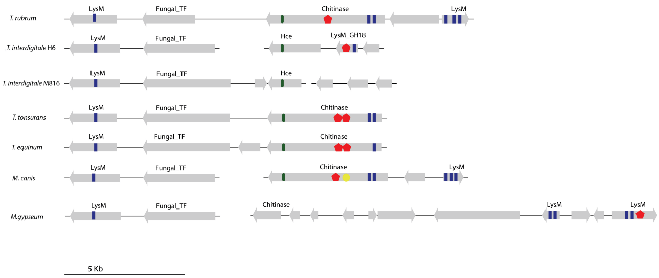
Figure S7. Variation in LysM-Hce gene cluster across sequenced Dermatophytes. In T. rubrum , the LysM-Hce gene is closely linked to two other LysM genes; this organization is most similar to that found in M. canis , although these genes are located on two different scaffolds.
