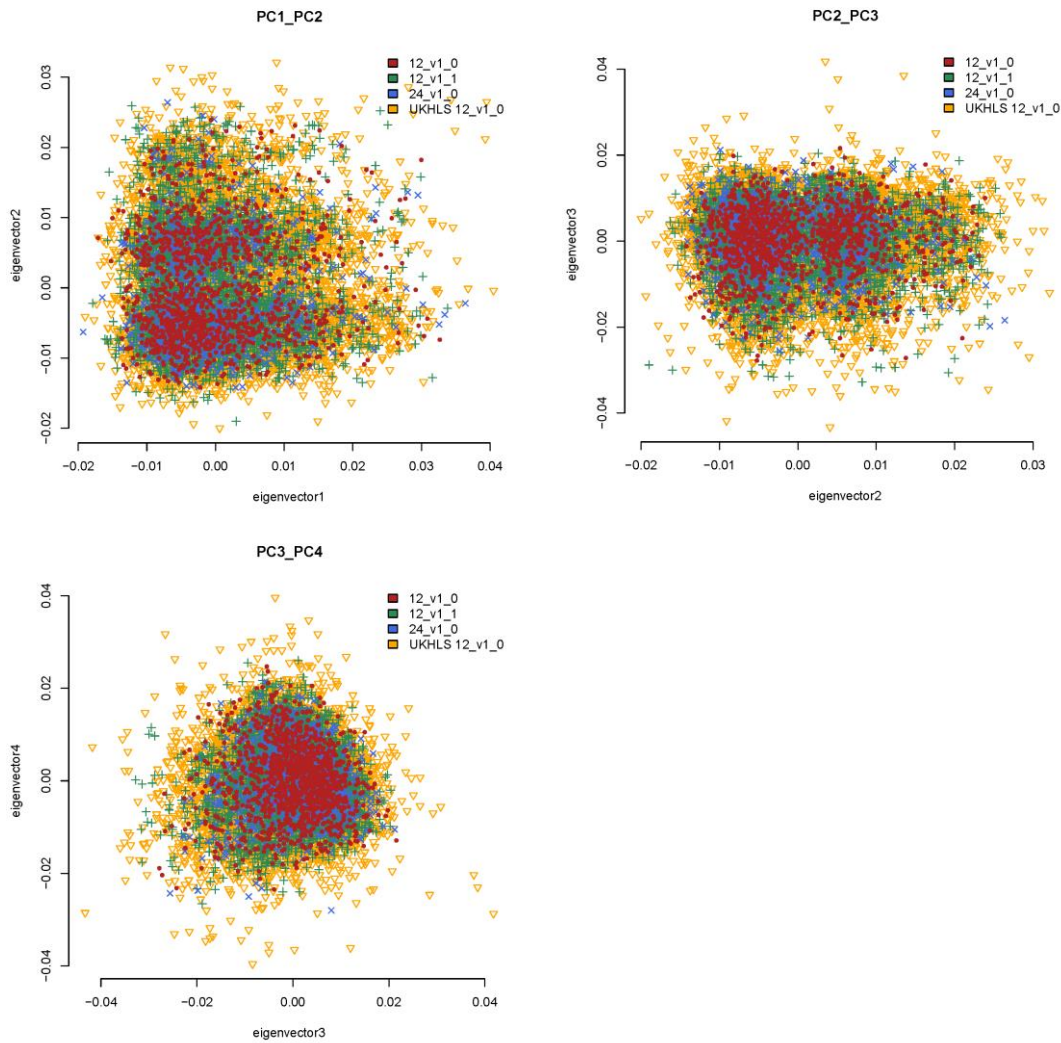
Figure S3. Plots of the first 4 principal components (PCs) from the principal component analysis of arcOGEN and UKHLS samples genotyped in the three different versions of the CoreExome chip after excluding complex regions. Cases genotyped in 12-sample arrays version 1.0 (12-v1.0) are in red; cases genotyped in 12-sample arrays version 1.1 (12-v1.1) are in green; cases genotyped in 24-sample arrays version v1.0 (24-v1.0) are in blue; controls previously genotyped on version 12-v1.0 are in yellow.
