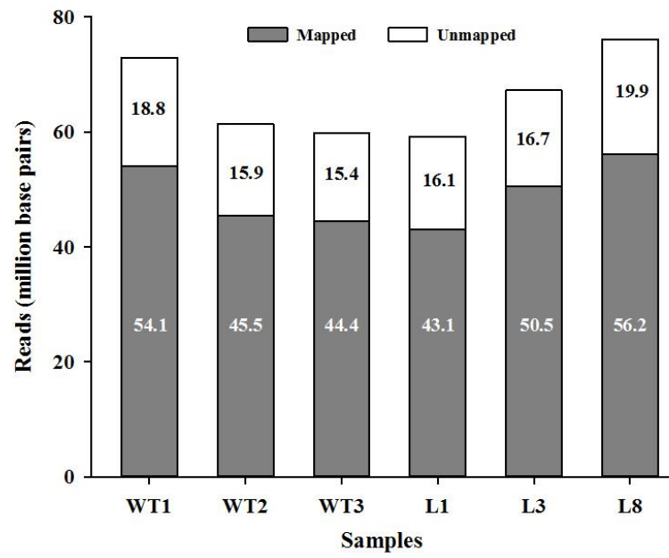
Figure S1. Total mapped and unmapped RNA-seq clean reads for transgenic lines and WT plants.
