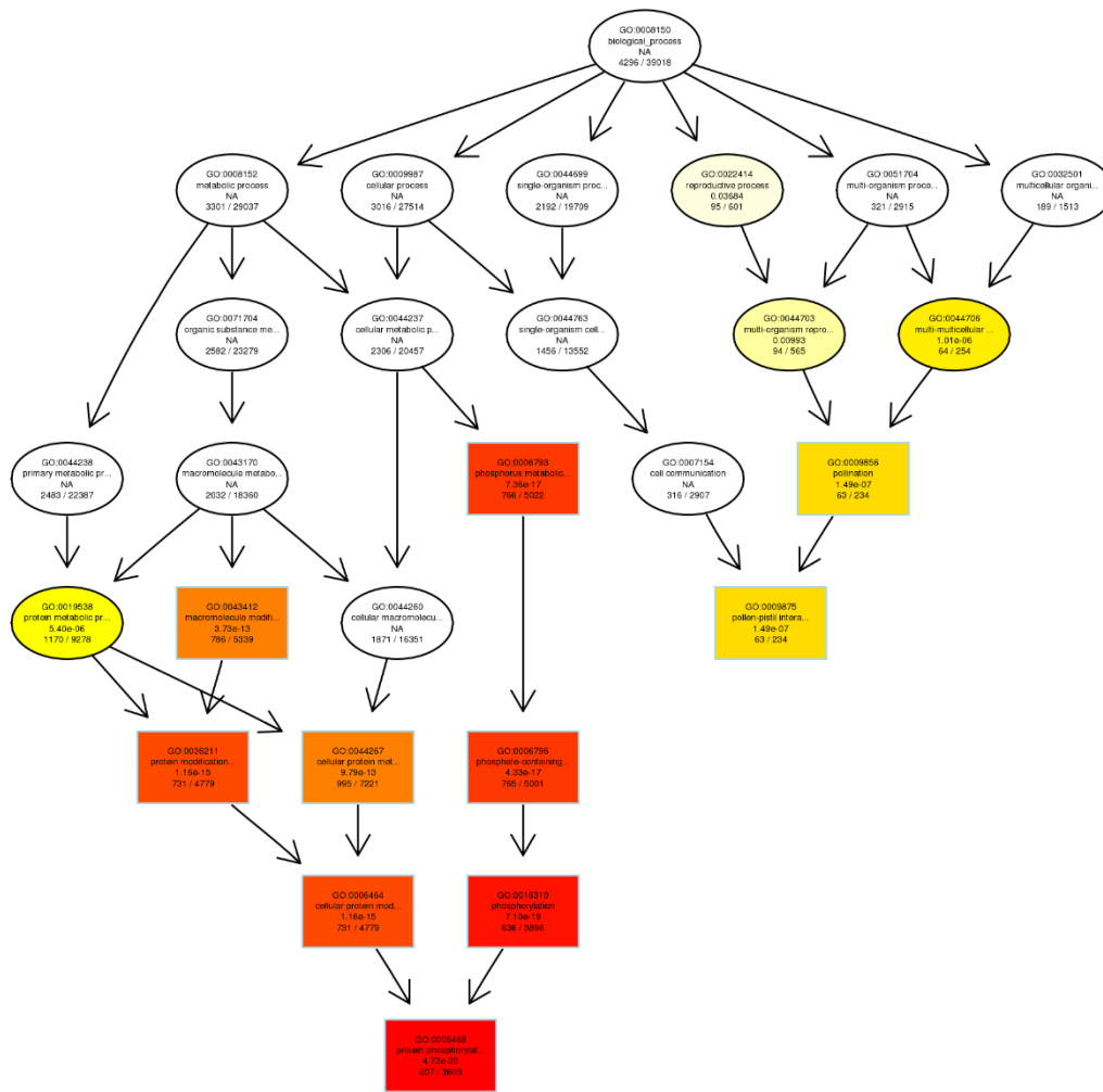
Figure S2. Enriched gene ontologies in differentially expressed genes of transgenic switchgrass. Each box shows the GO term number, the p-value in parenthesis, and GO term. Box colors indicates levels of statistical significance: yellow = 0.05; orange = e-05 ; and red = e-09 .
