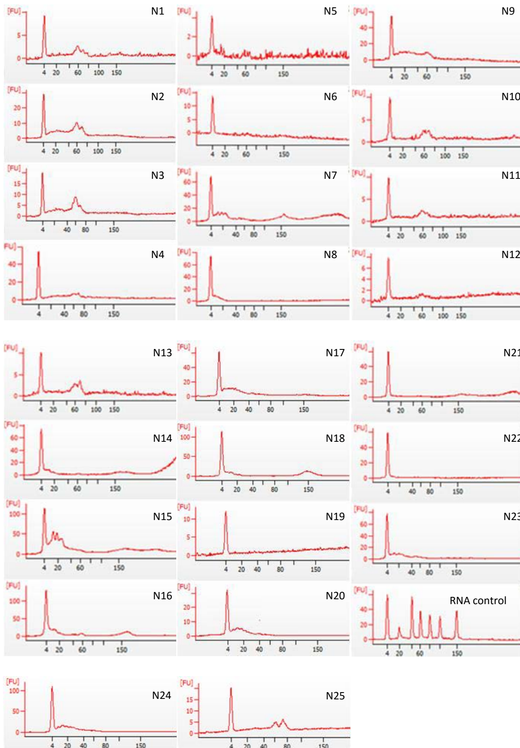
Supplemental Figure 1: Quality control of small RNA from plasma samples of normal control using Agilent 2100 bioanalyzer
