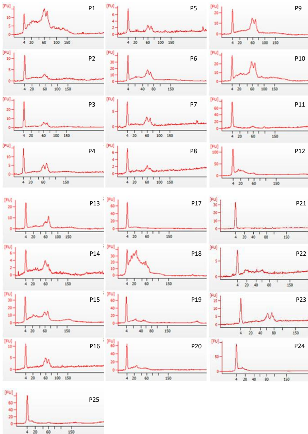
Supplemental Figure 2: Quality control of small RNA from plasma samples of PD patients using Agilent 2100 bioanalyzer
