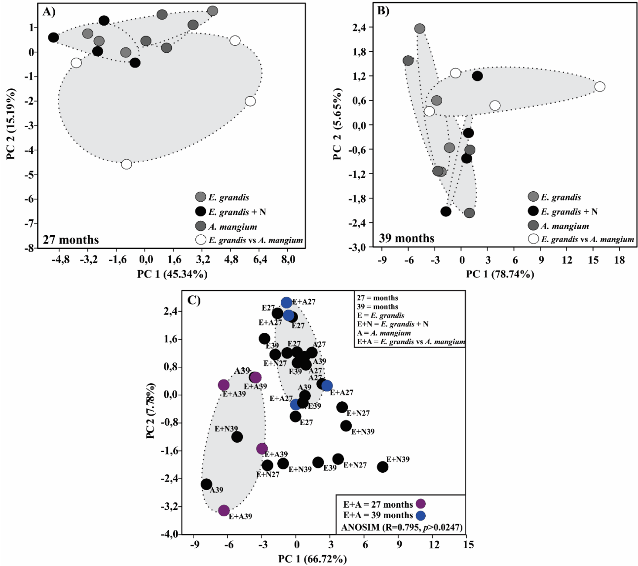
Supplementary Figure S2. Principal Coordinates Analysis (PCoA) based on the metabolic profile degradation of the soil microbial community accessed by Biolog EcoPlates in pure and mixed E. grandis and A. mangium plantations. A) 27 and B) 39 months after planting, and C) total profile.
