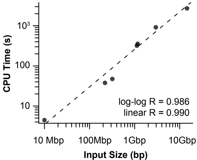
K-mer kernel
