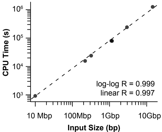
Alignment kernel
