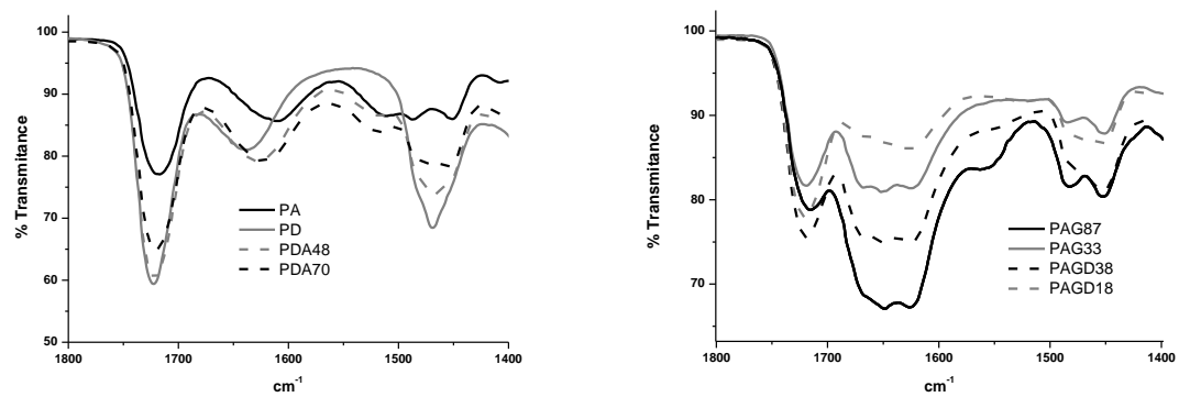
Fig S1. FTIR spectrums of the synthesized (co)polymers Pa, PD, PDA48 and PDA70 (left graph) and the guanylated polymers PAG87, PAG33, PAGD38 and PAGD18 (right graph).
