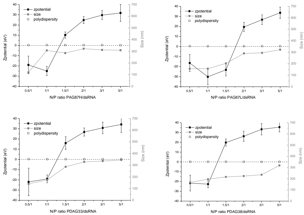
Fig S3. Size and Z potential results for the polyplexes formed with PAG87H, PAG87L, PDAG33 and PDAG38
