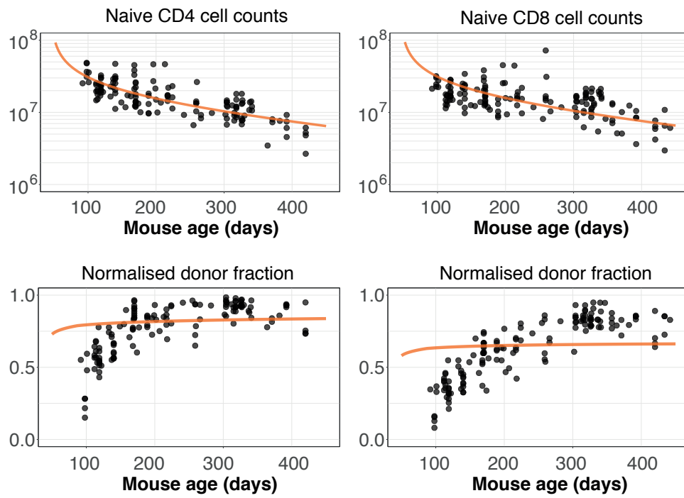
Figure S1: The density-dependent model fails to explain the replacement kinetics in busulfan chimeras. Data are as in Fig 3 in the main text.
