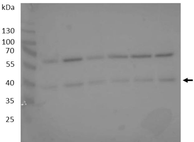
p-p38 Thr180/Tyr182
