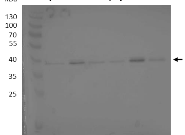
p-ERK Thr202/Tyr204
