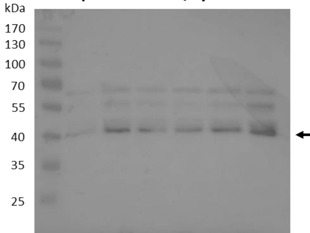
p-JNK Thr183/Tyr185
