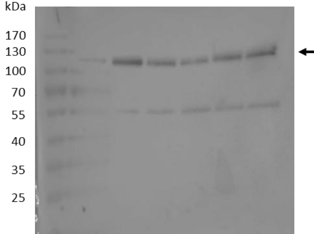
p-PKD Ser744/Ser748
