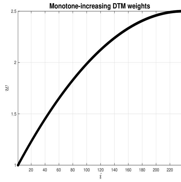
Fig. S2. DTM weights w_{iS} used in the computation of \tilde{\eta} .
