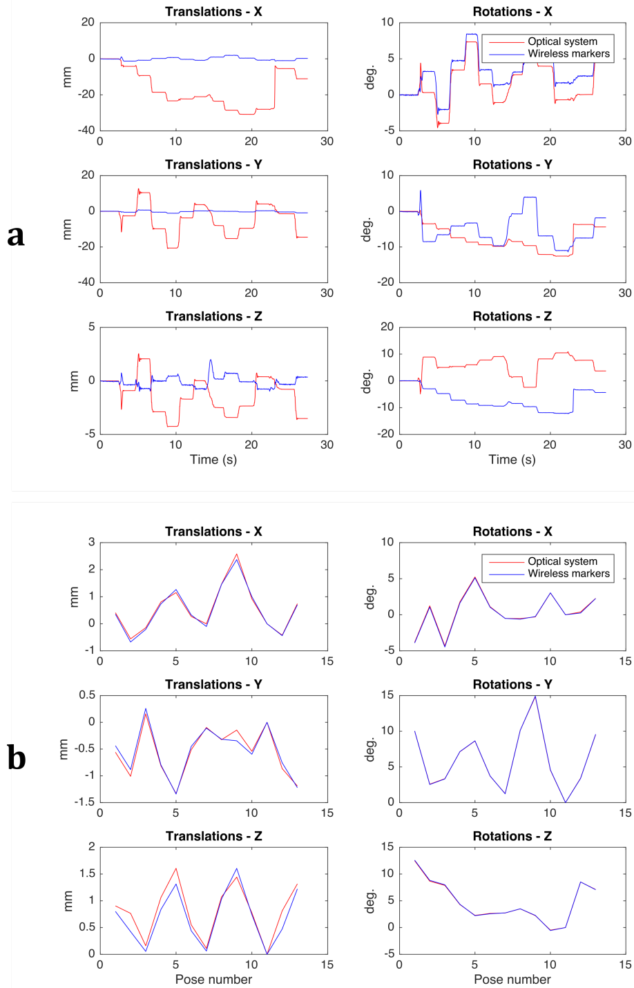
Figure S1: Result of a single calibration experiment: (a) plot of raw data collected from optical system (red curves) and wireless markers (blue curves), relative to the first position; (b) extracted poses from both the optical system and wireless markers; the optical data have been transformed to the MRI scanner reference frame using the calculated cross-calibration matrix T_{CS} .
