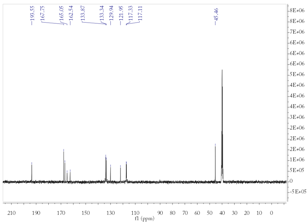
The spectra of 1 H and 13 C NMR of compound 1j
