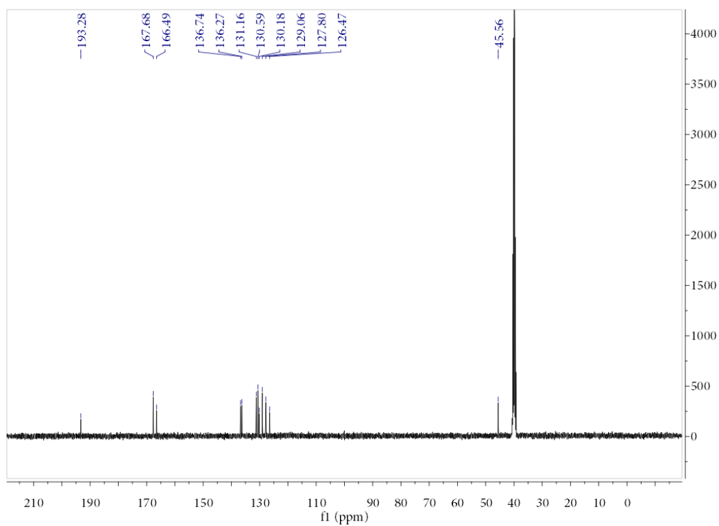
The spectra of ^1\text{H} and ^{13}\text{C} NMR of compound 1i
