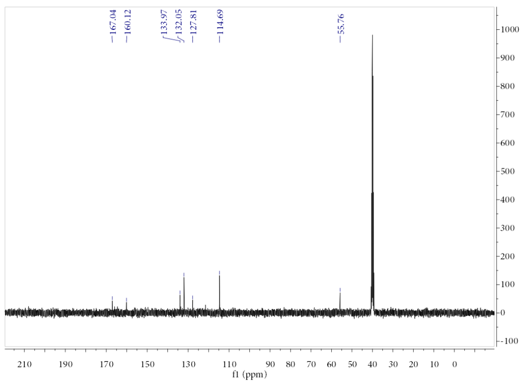
The spectra of ^1\text{H} and ^{13}\text{C} NMR of compound 3a
