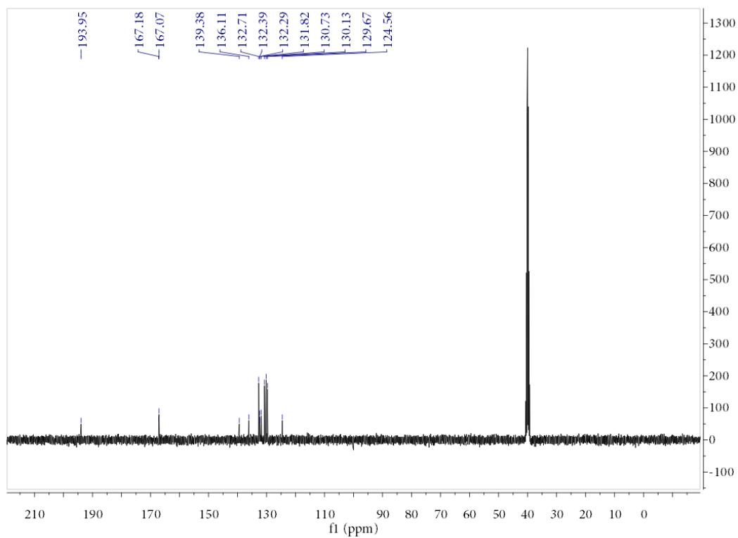
The spectra of 1 H and 13 C NMR of compound 2h
