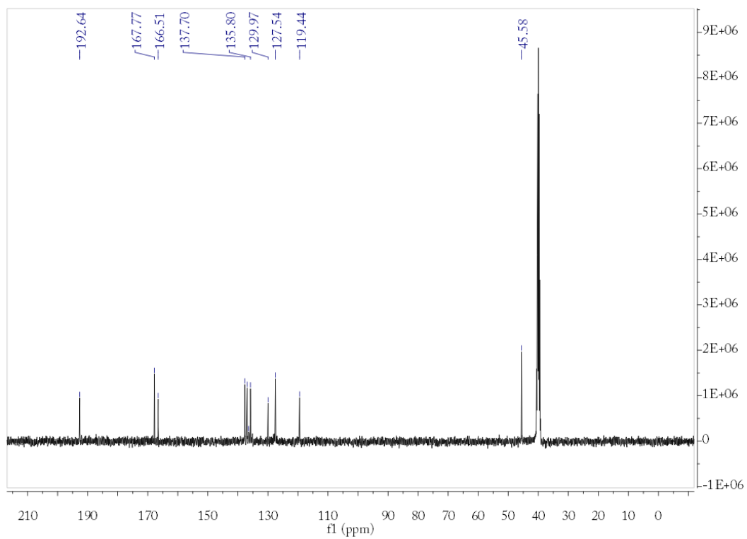
The spectra of 1 H and 13 C NMR of compound 1c
