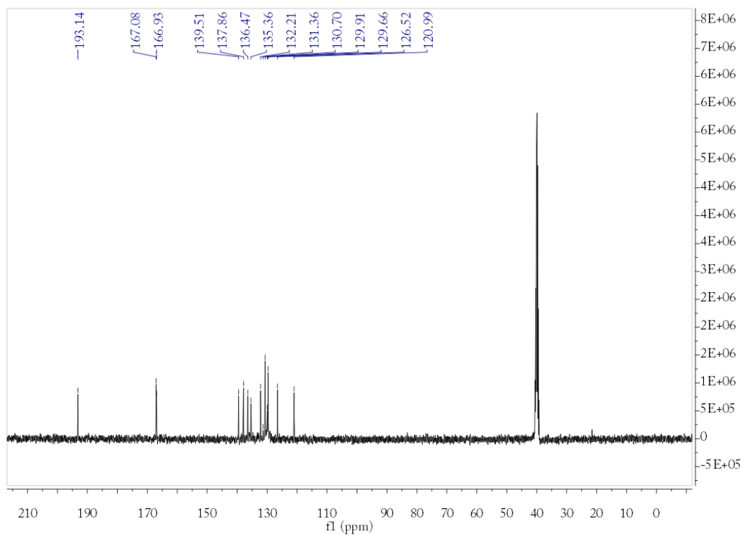
The spectra of ^1\text{H} and ^{13}\text{C} NMR of compound 2c
