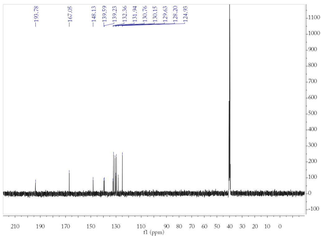
The spectra of ^1\text{H} and ^{13}\text{C} NMR of compound 2I
