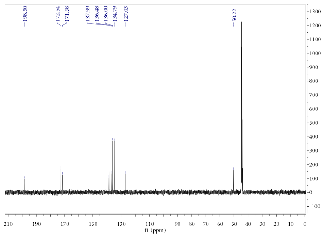
The spectra of 1 H and 13 C NMR of compound 1a
