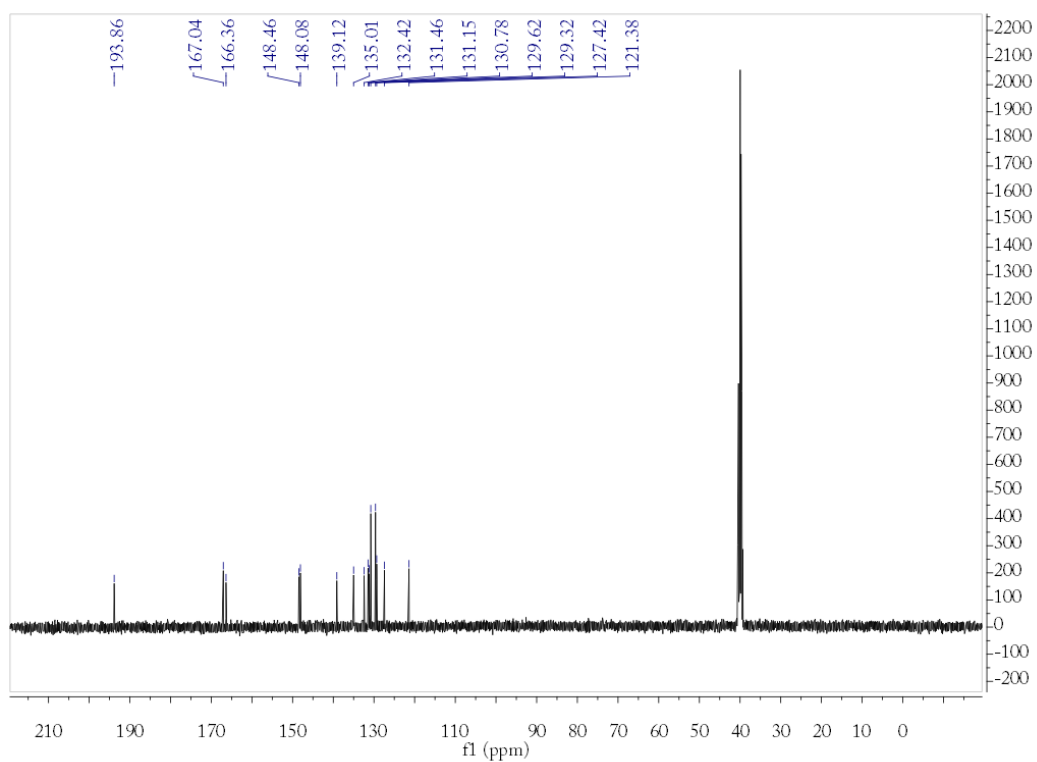
The spectra of ^1\text{H} and ^{13}\text{C} NMR of compound 2m
