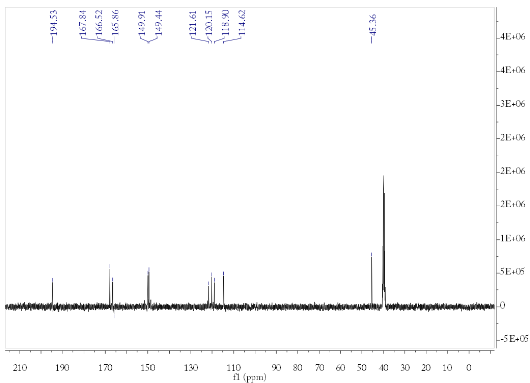
The spectra of 1 H and 13 C NMR of compound 1b
