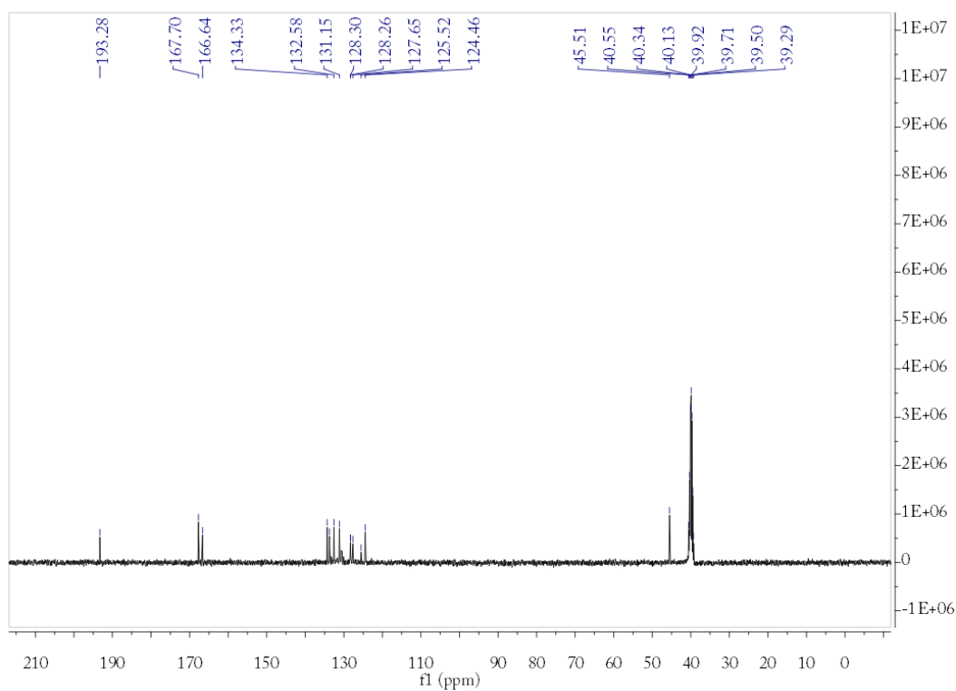
The spectra of ^1\text{H} and ^{13}\text{C} NMR of compound 1k
