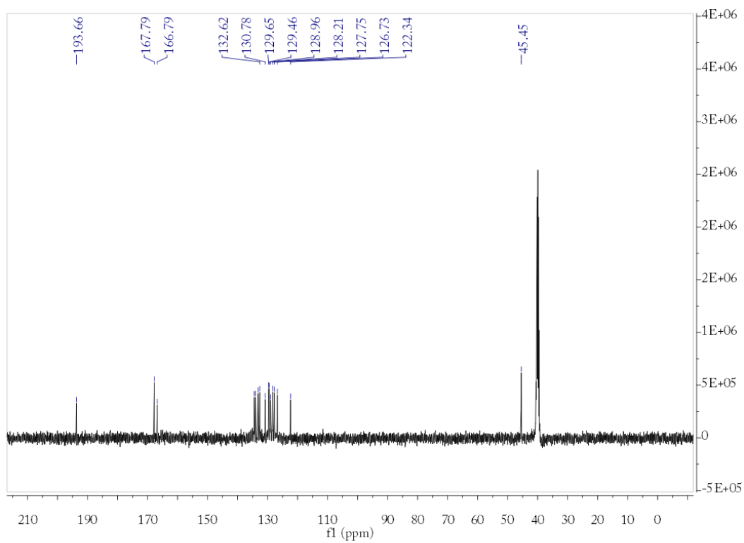
The spectra of ^1\text{H} and ^{13}\text{C} NMR of compound 1f
