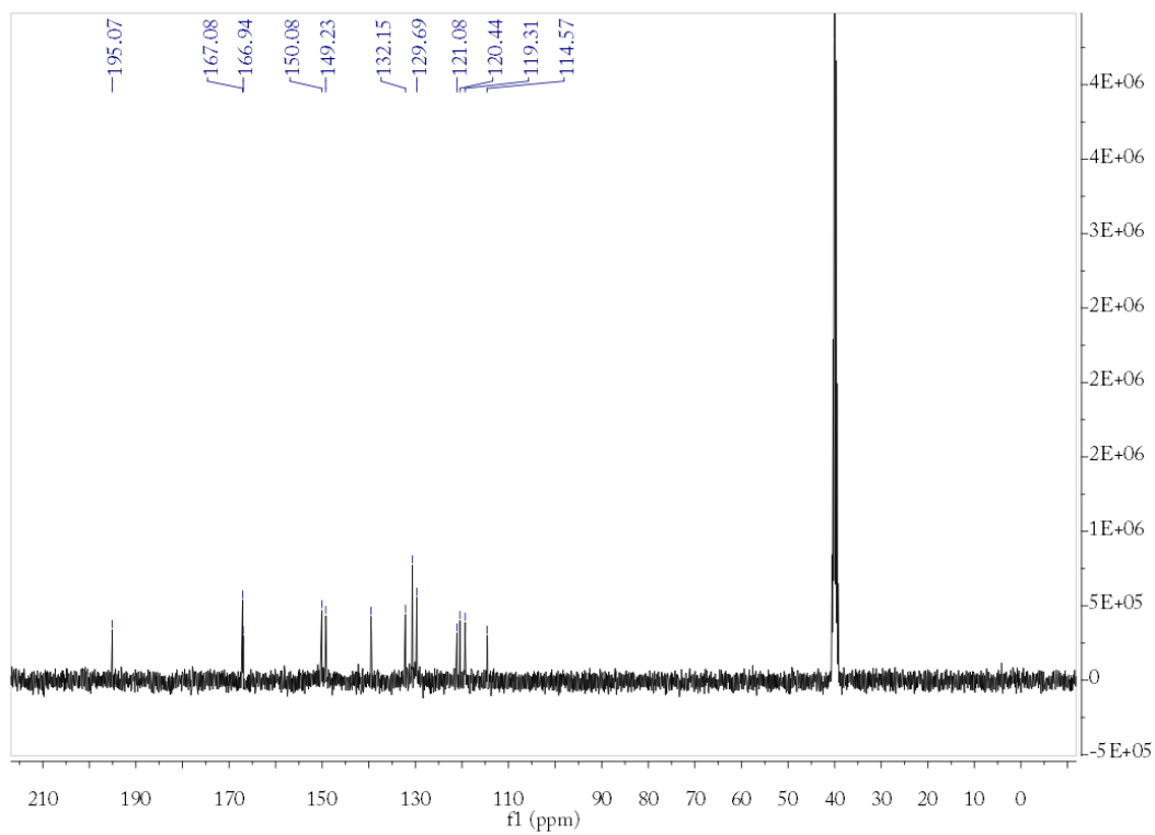
The spectra of ^1\text{H} and ^{13}\text{C} NMR of compound 2b
