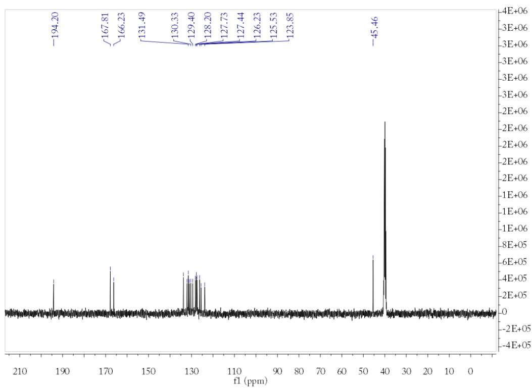
The spectra of ^1\text{H} and ^{13}\text{C} NMR of compound 1e
