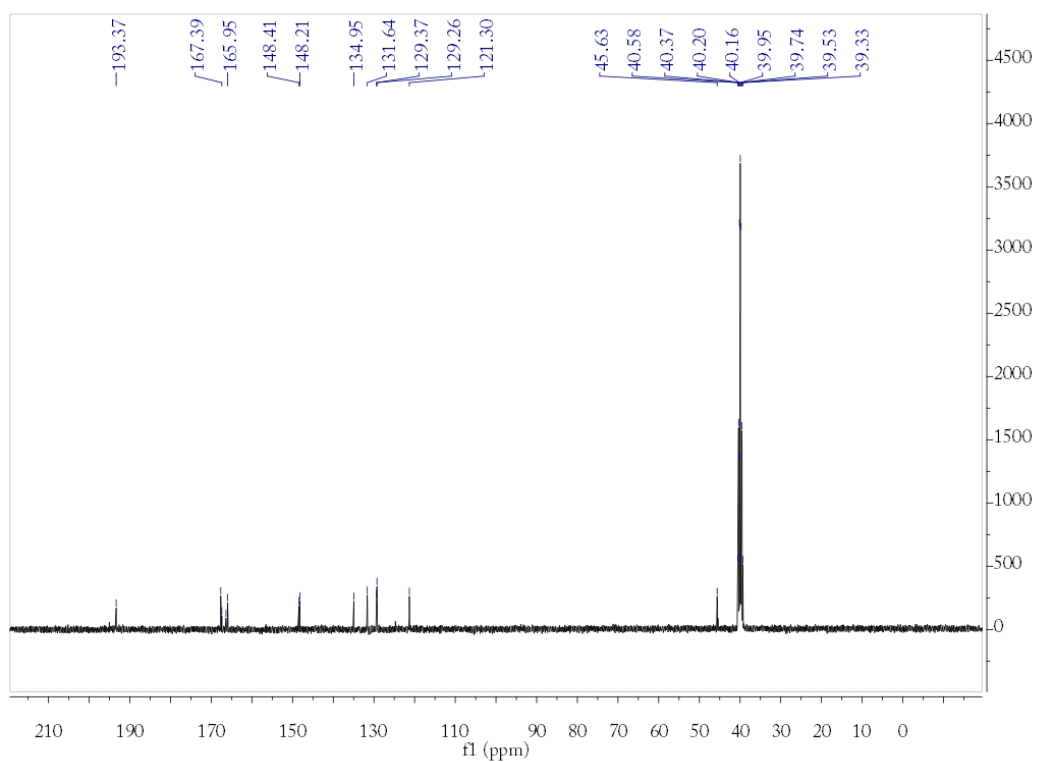
The spectra of 1 H and 13 C NMR of compound 1m
