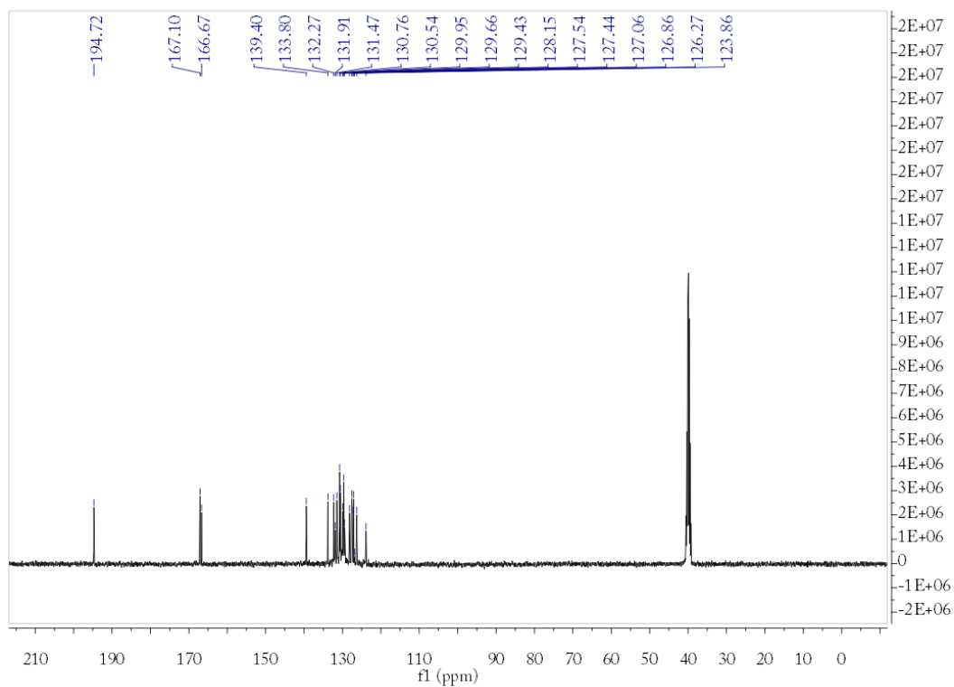
The spectra of 1 H and 13 C NMR of compound 2e
