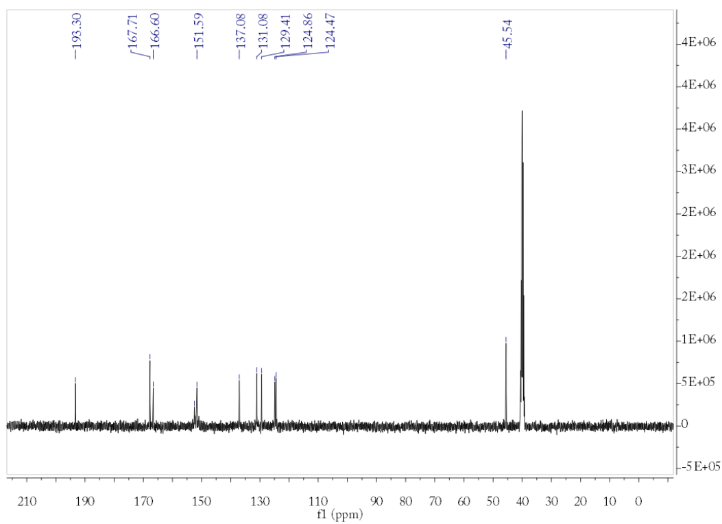
The spectra of ^1\text{H} and ^{13}\text{C} NMR of compound 1d
