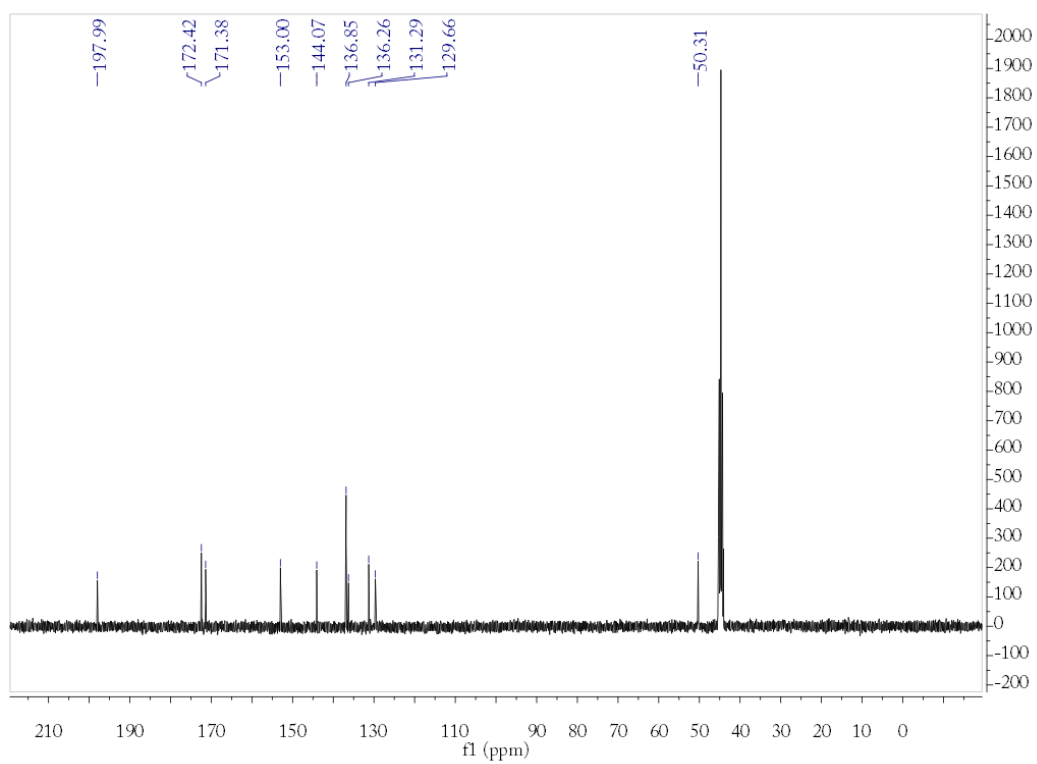
The spectra of ^1\text{H} and ^{13}\text{C} NMR of compound 11
