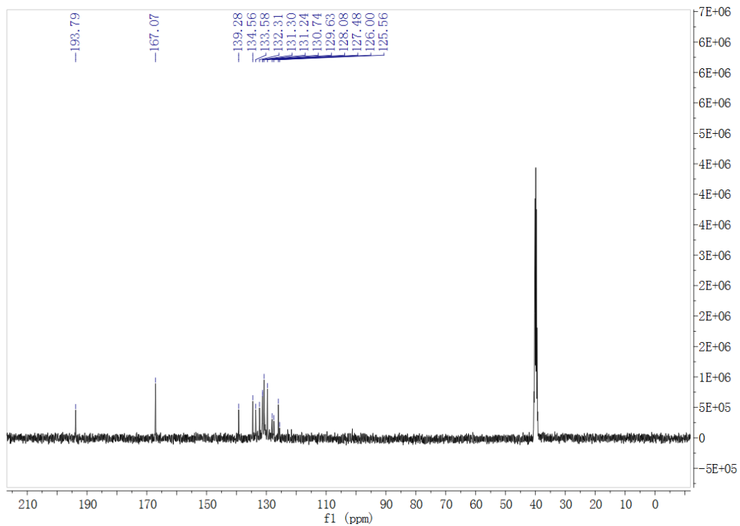
The spectra of ^1\text{H} and ^{13}\text{C} NMR of compound 2k
