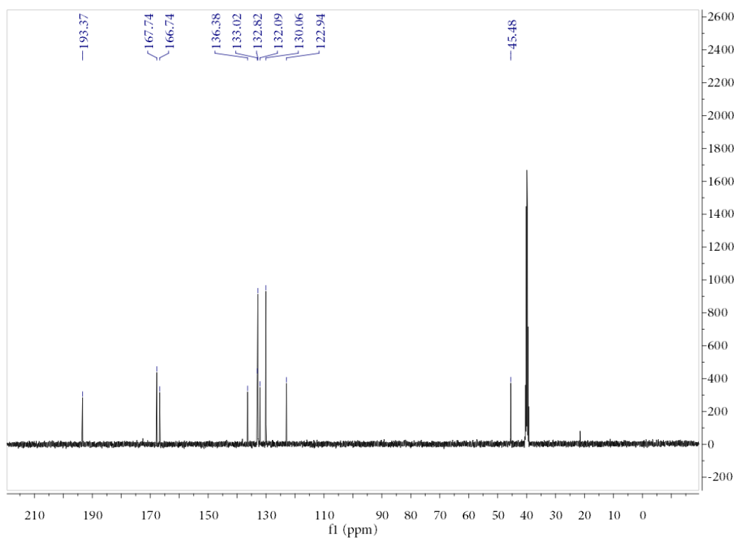
The spectra of ^1\text{H} and ^{13}\text{C} NMR of compound 1h
