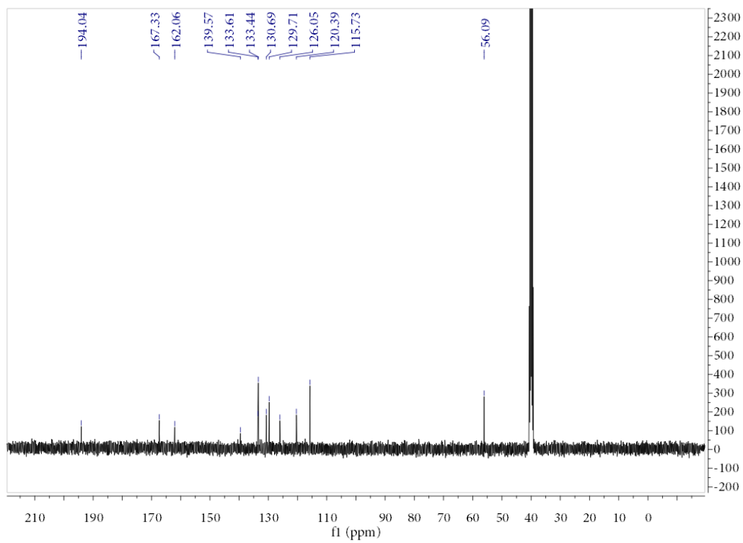
The spectra of ^1\text{H} and ^{13}\text{C} NMR of compound 2g
