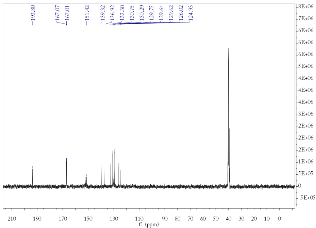
The spectra of ^1\text{H} and ^{13}\text{C} NMR of compound 2d
