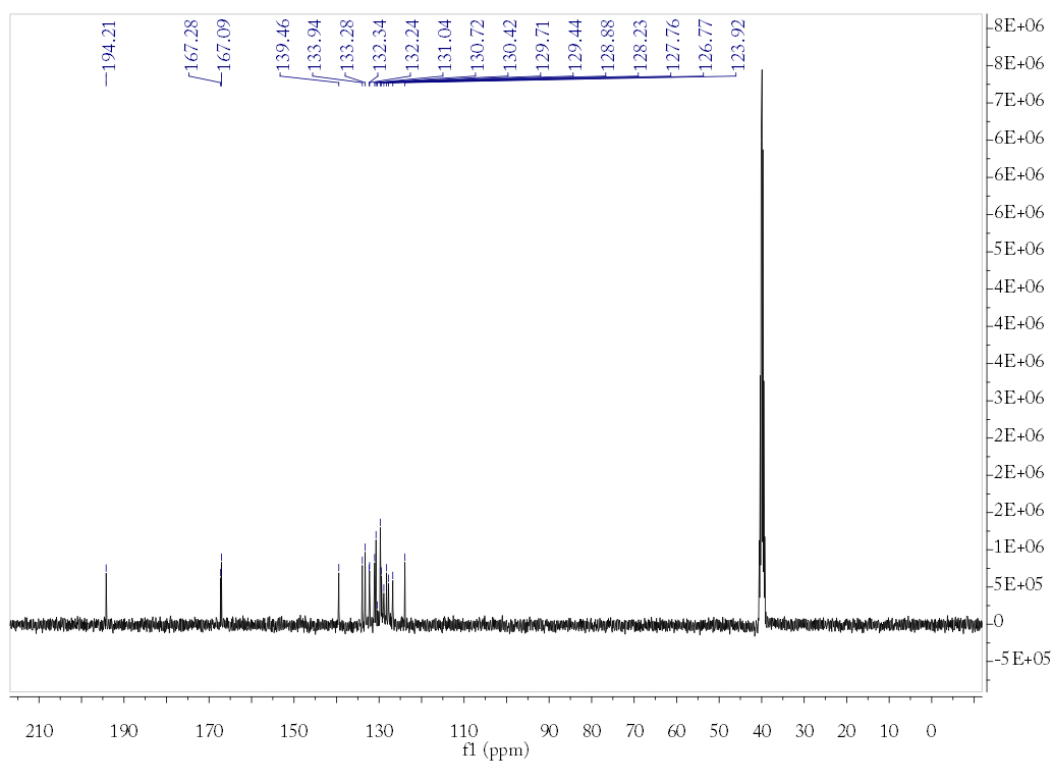
The spectra of 1 H and 13 C NMR of compound 2f
