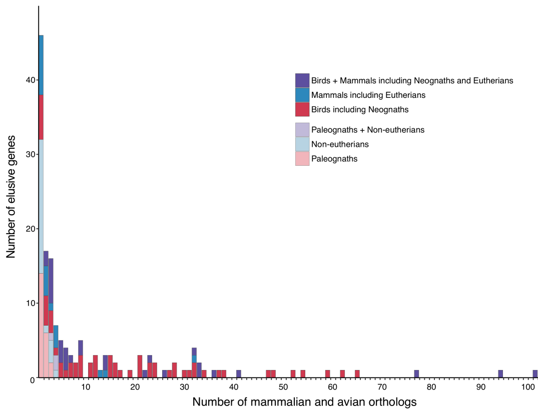
Figure S11. Frequency distribution of the elusive genes relating to number of the mammalian and avian orthologs
