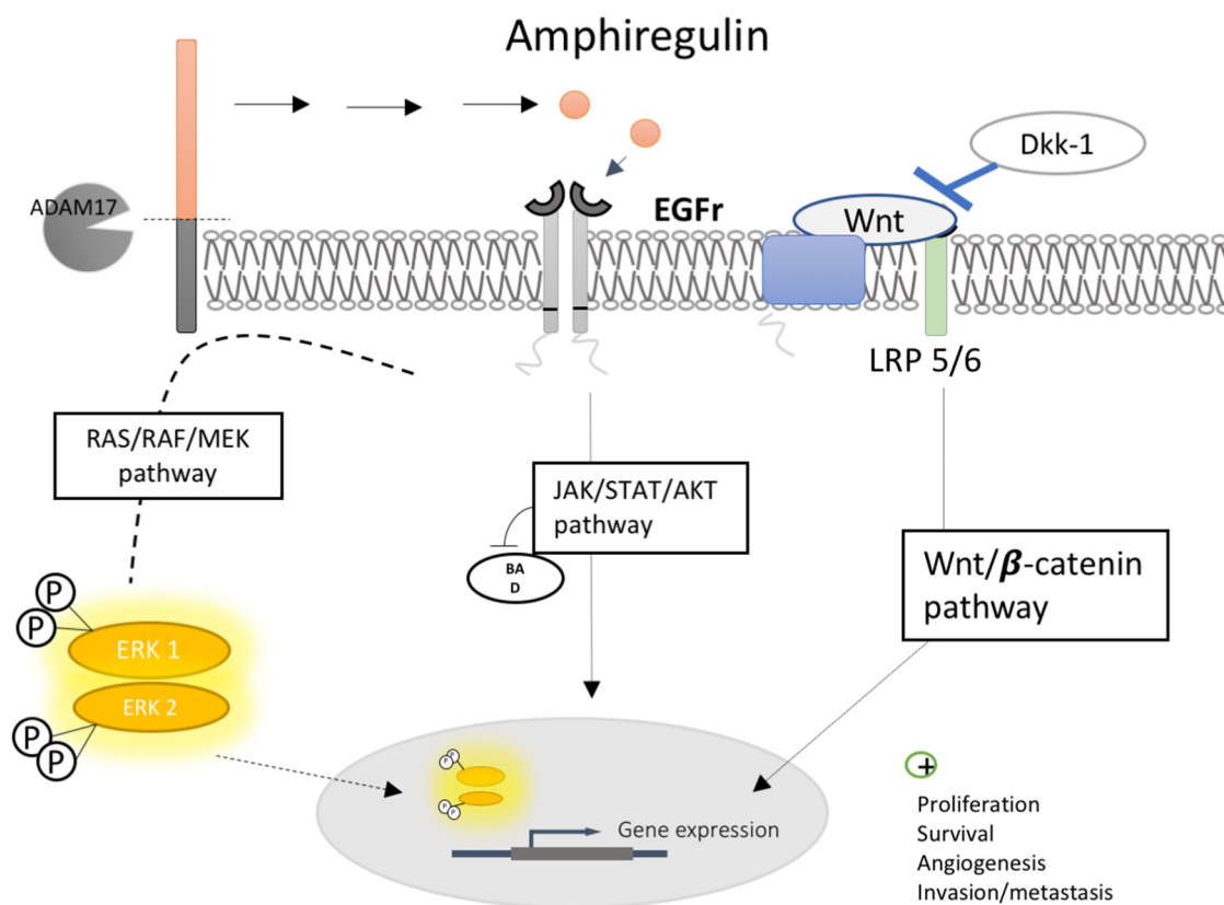
Supplementary Figure 1: Overview of amphiregulin activation of the MAP kinase pathway.
