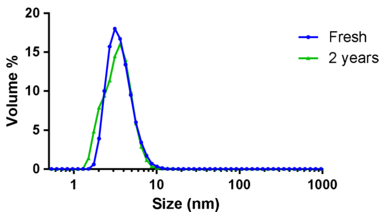
Figure S1. Hydrodynamic particle size of 40mM CHAT in water (as per conditions of synthesis), when freshly prepared and when 2 years old by Dynamic Light Scattering.
