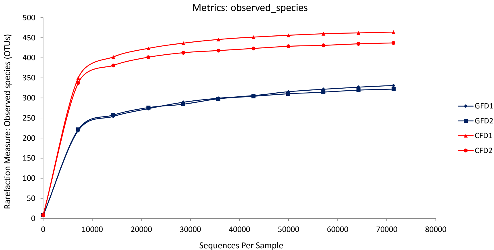
Supplementary Figure 1: Rarefaction curves of observed species (OTUs) number clustered at 3% 16S rRNA sequences variations generated from D. rerio fed with control formulated diet (CFD) and gluten formulated diet (GFD). This graph was created by QIIME (ver.1.8.0) by plotting the number of OTUs against the number of sequences. The plateau of the curves indicates that most of the species were observed in all four samples.
