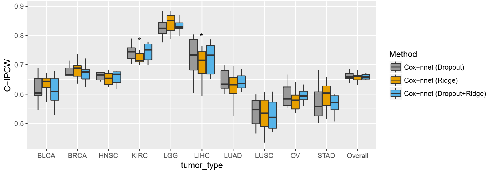
C-IPCW performance
