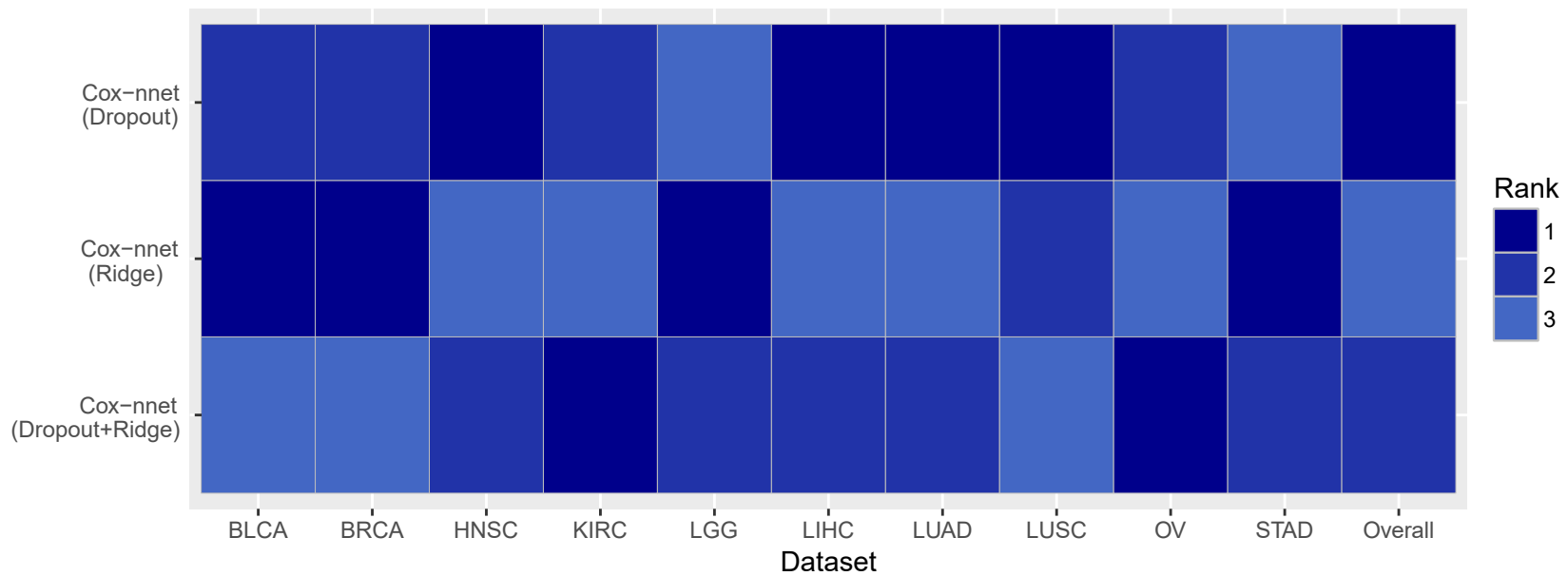
C-IPCW performance
