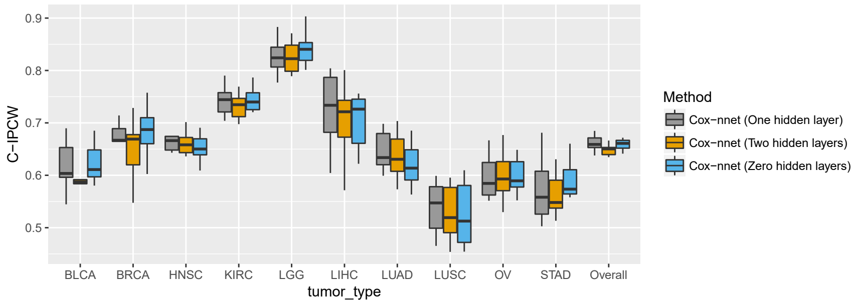
C-IPCW performance
