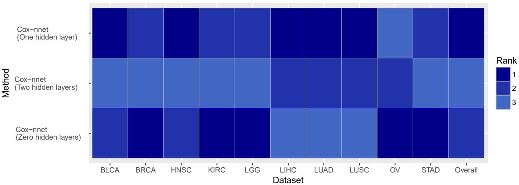
C-IPCW performance
