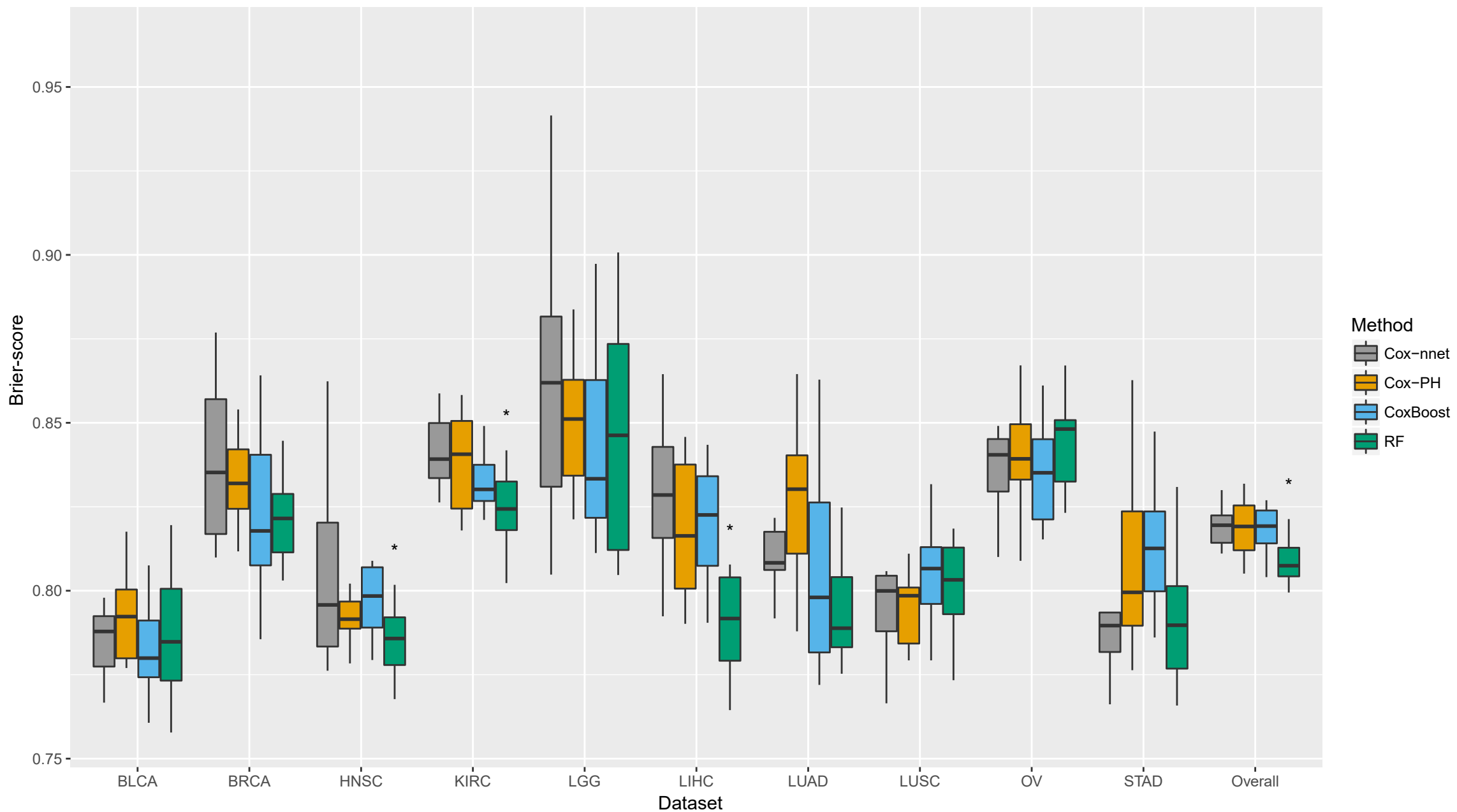
Performance across TCGA datasets (Brier-score)
