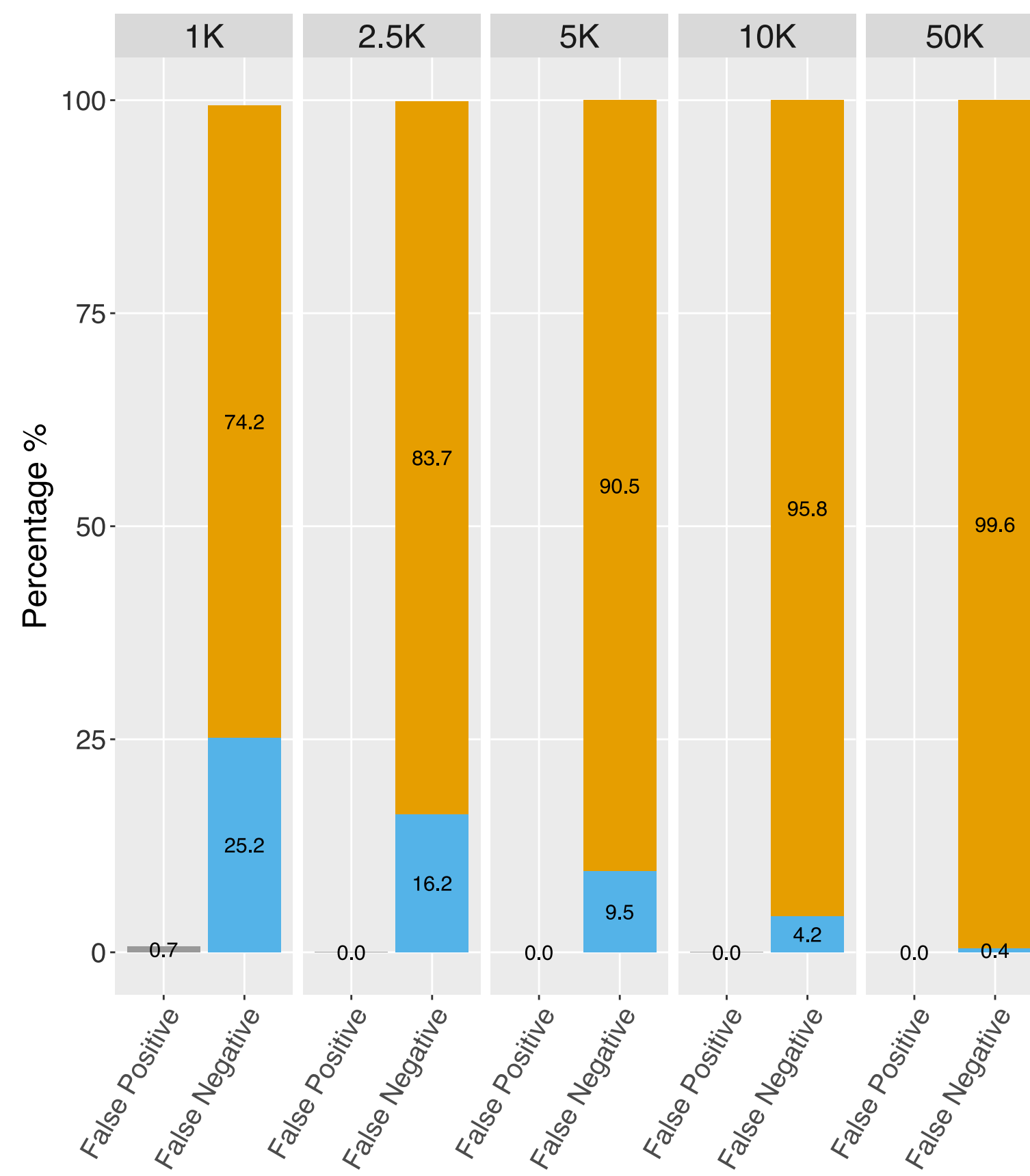
20% allelic error
