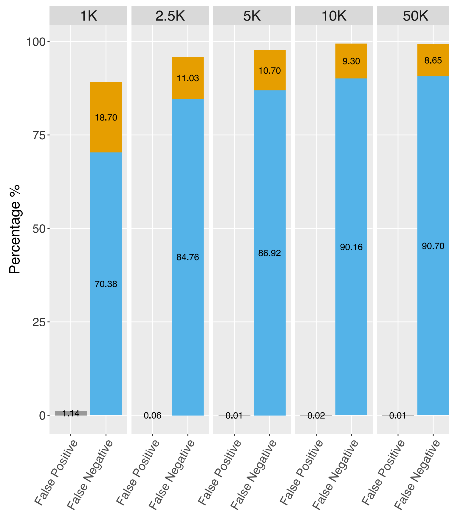
20% allelic error
