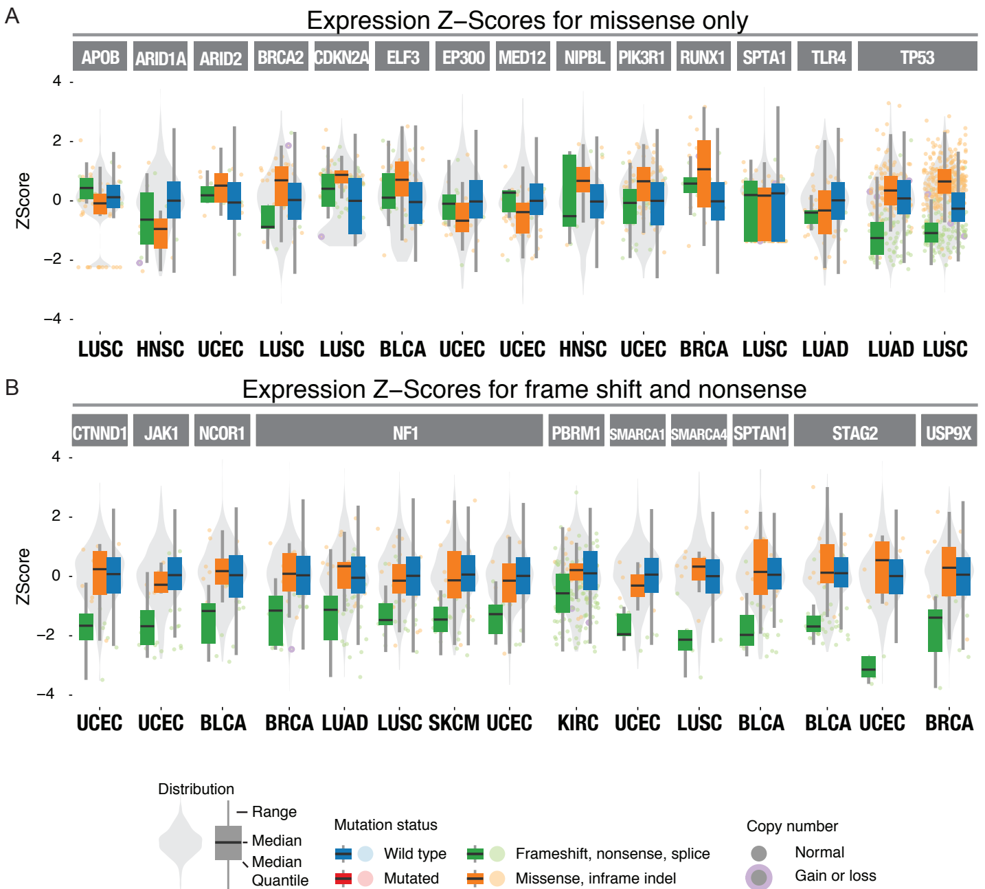
Figure S2: Alternative grouping for cis-expression differences. Related to Figure 4. For the main text Figure 4, only missense mutations and frameshift indels were considered. The top 15 t-values using an extended definition of missense mutations to include in-frame indels A. And frameshift/nonsense mutations, here, include splice site mutations B.
