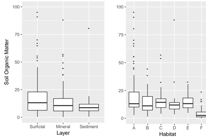
S2 Figure. Boxplots of SOM (g/kg) contents measures at all sites compared across layers and habitats.
