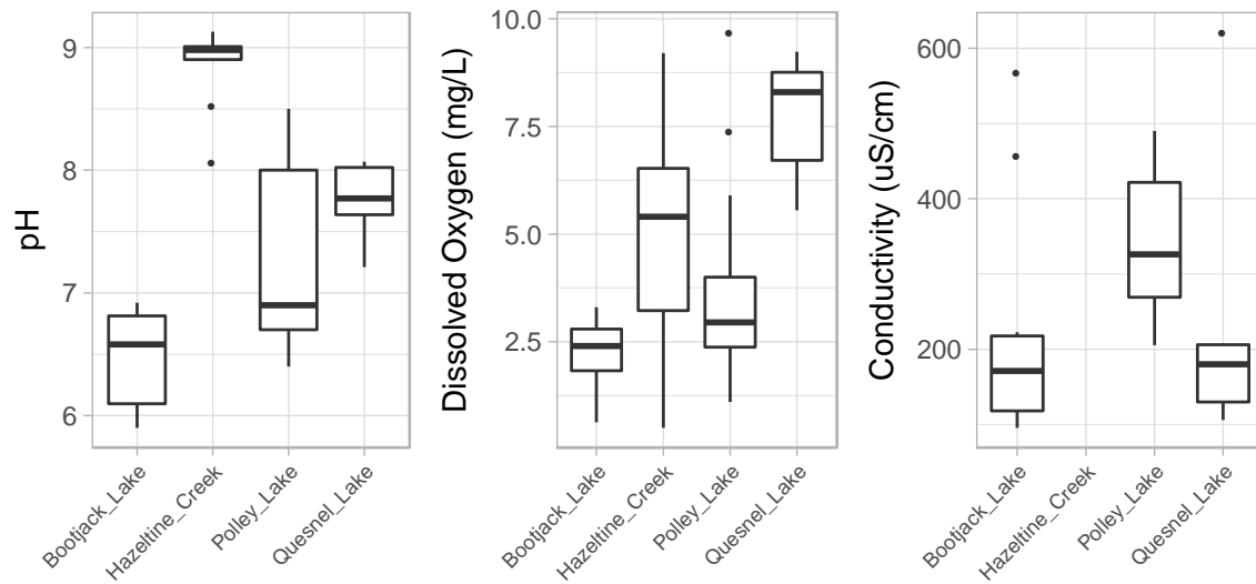
S4 Figure. Pore water pH, dissolved oxygen (mg/L) and conductivity ( \mu\text{S}/\text{cm} ). Box-whisker plots reflect medians, quartiles and outliers by lake/stream.
