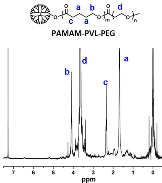
Figure S1. 1 H NMR spectrum of PAMAM-PVL-PEG.
