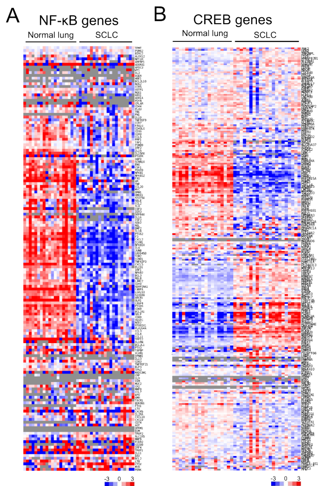
Supplementary Figure S4. NF- \kappa B and CREB activity in human SCLC samples. Human SCLC RNAseq data were kindly shared by Dr. Seshagiri group ( Nat. Genet. 2012. 44 :1111-1116). Heatmap of the expression values of 153 NF- \kappa B target genes ( A ) and 264 CREB target genes ( B ) in normal lungs and SCLC primary tumors was shown.
