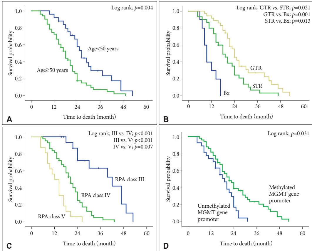
Supplementary Fig. 1. Kaplan-Meier survival curves according to the other meaningful factors associated with overall survivals. A: age (<50 years vs. ≥50 years). B: extent of resection (STR vs. GTR vs. Bx). C: RPA class (III vs. IV vs. V). D: methylation status of MGMT gene promoter (methylated vs. unmethylated). STR, subtotal resection; GTR, gross total resection; Bx, biopsy; RPA, recursive partitioning analysis; MGMT, O6-methyl guanine DNA methyltransferase.
