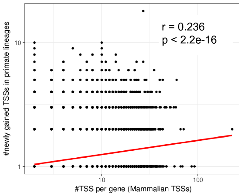
Supplemental Figure S11 Relationship between the number of old (‘mammalian’) TSSs per gene and the number of newly gained TSSs in primate lineages, on a \log_{10} scale. The red line is derived from linear regression based on the data points. Pearson’s r and the corresponding p -value are also shown in the figure.
