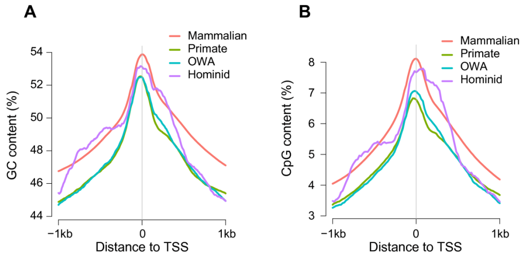
Supplemental Figure S2 Comparison of GC content (A) and CpG content (B) between four groups.
