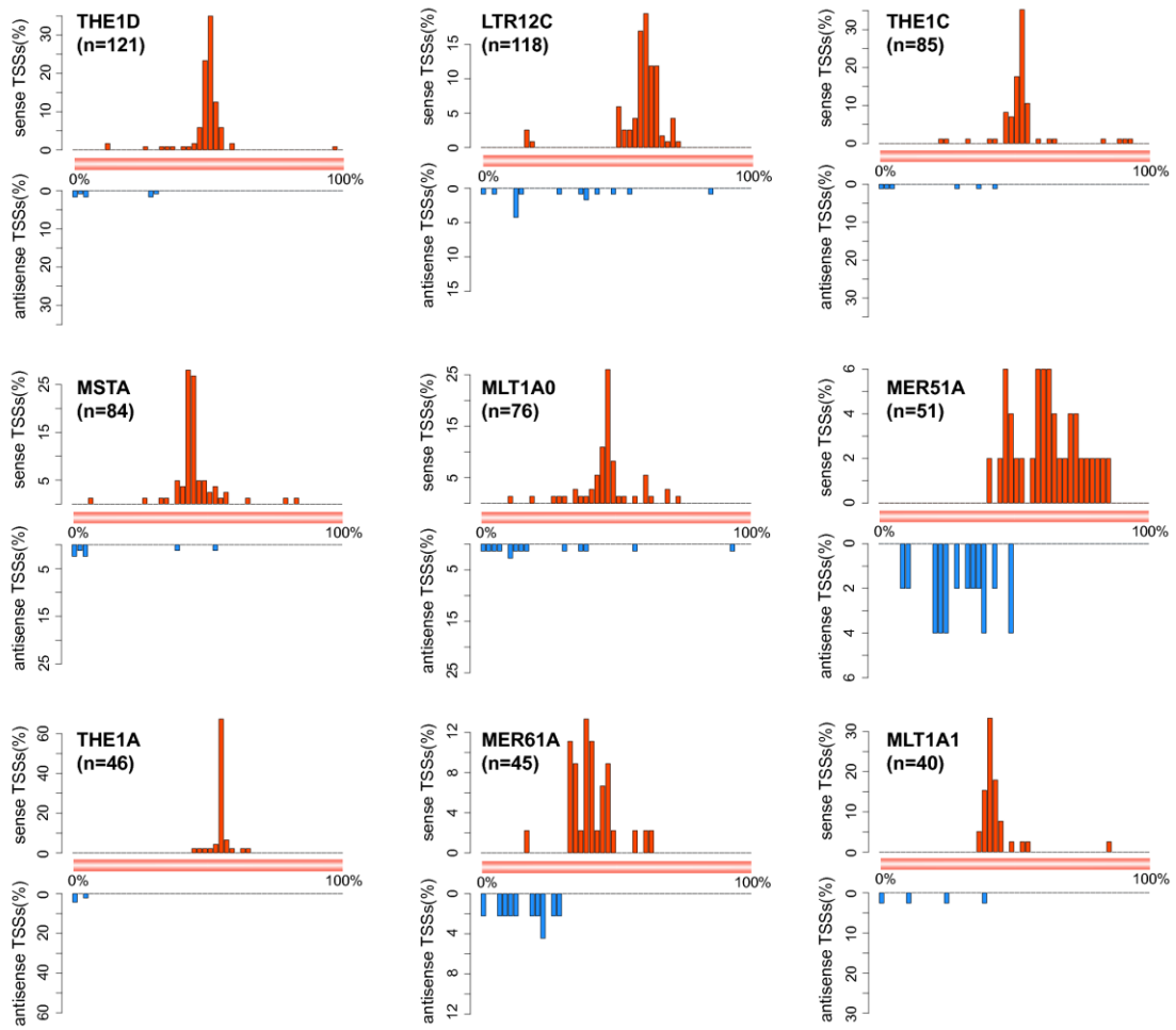
Supplemental Figure S5 Distribution of young TSSs along LTR subfamilies. These nine subfamilies are among the top 10 LTR subfamilies which harbor most young TSSs. The tenth, THE1B, has already been shown in Fig. 2b . Number of young TSSs for each subfamily is given in the bracket.
