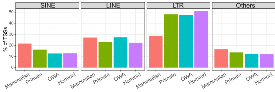
Supplemental Figure S6 Percentages of TSSs associated with different retrotransposons which contain a TATA-box motif starting at 25-35 bp upstream regions of the dominant TSSs.
