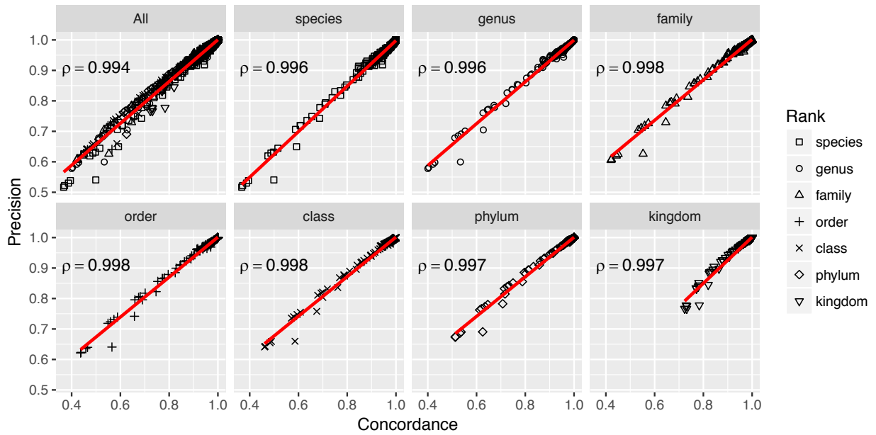
Supplemental Figure S10 | Classification Concordance versus Precision. Per rank correlation between paired-end classification concordance and precision on 55 simulated datasets, based on taxMaps, Kraken, MegaBLAST, Centrifuge and BLASTN single-end classification. For each rank, the corresponding Spearman's rank correlation coefficient \rho is indicated.
