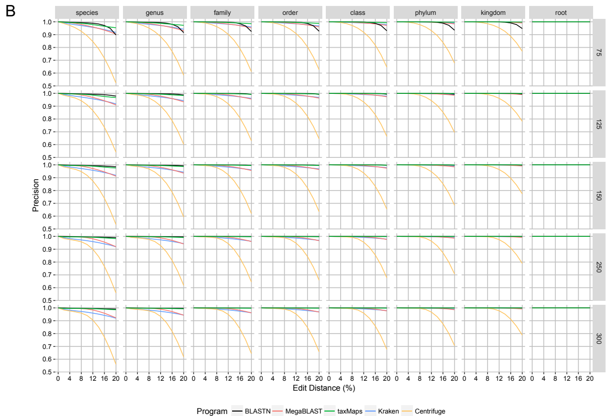
Supplemental Figure S3 | Classification accuracy and performance on simulated metagenomics paired-end datasets. Classification (A) sensitivity and (B) precision as function of average sequence divergence and read length for all the major taxonomic ranks.
