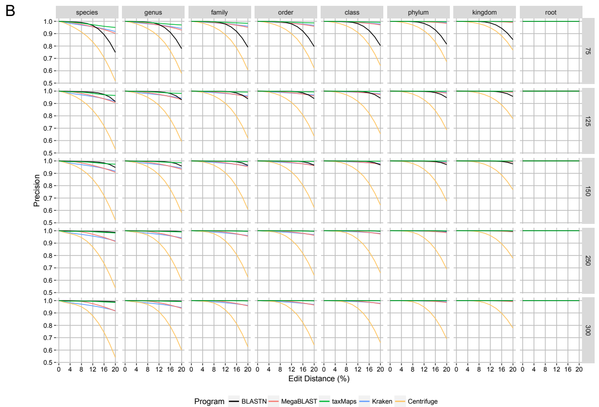
Supplemental Figure S4 | Classification accuracy and performance on simulated metagenomics single-end datasets. Classification (A) sensitivity and (B) precision as function of average sequence divergence and read length for all the major taxonomic ranks.
