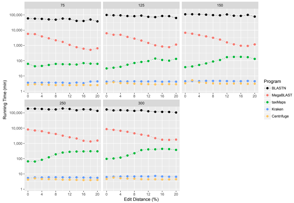
Supplemental Figure S5 | Classification speed on simulated datasets. Wall clock time required for the classification of 55 simulated datasets, each consisting of 10M read-pairs of varying length (indicated at the top of each panel), as a function of average sequence divergence.
