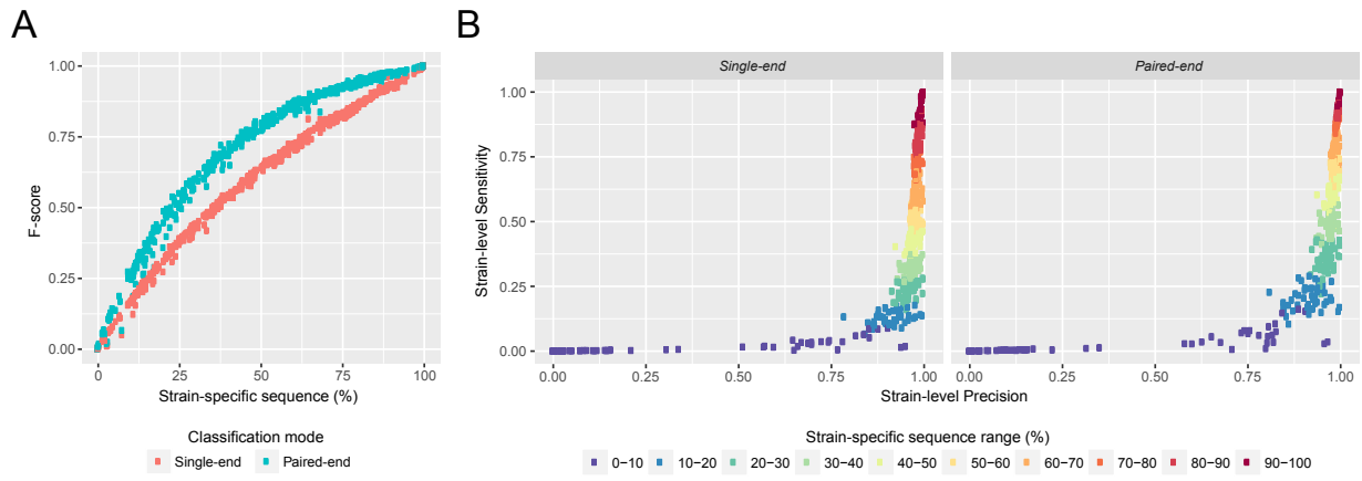
Supplemental Figure S6 | taxMaps strain-level classification accuracy using single-end and paired-end modes. (A) taxMaps strain-level classification F-score for 500 bacterial genomes, as a function of the percentage of strain-specific sequence. (B) taxMaps strain-level classification sensitivity and precision for the same set of genomes.
