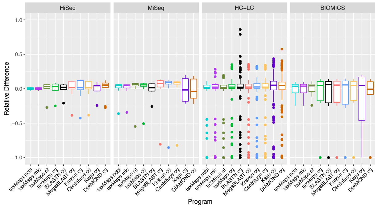
Supplemental Figure S9 | Relative difference between estimated and real genus abundance on 4 mock metagenomics communities. Genus abundance has been directly estimated from taxonomic classification by different tools and by making use of different indexes in taxMaps.
