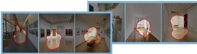
Cluster 5
