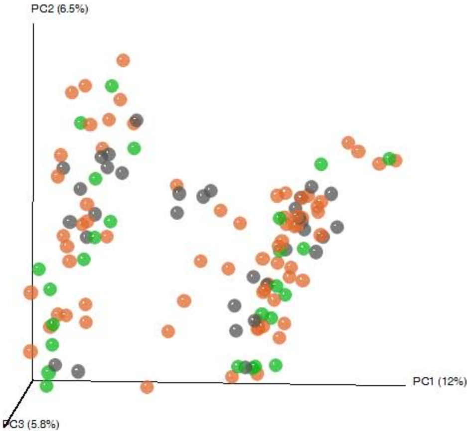
Unweighted UniFrac
