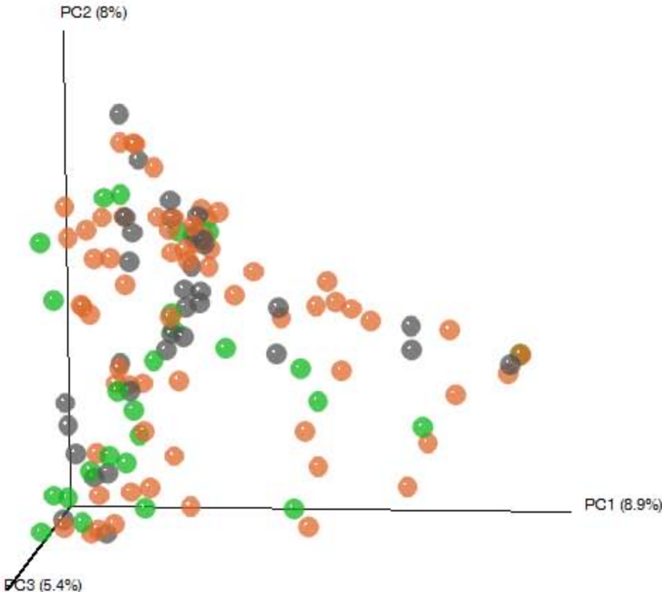
Bray-Curtis
