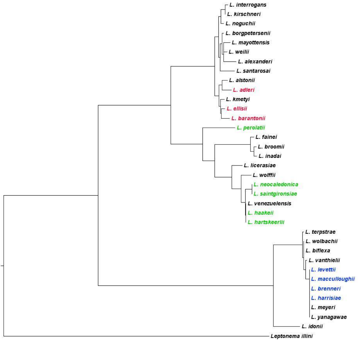
Supplementary Figure 2: 16S rRNA phylogeny of the Leptosira genus with novel species in color
