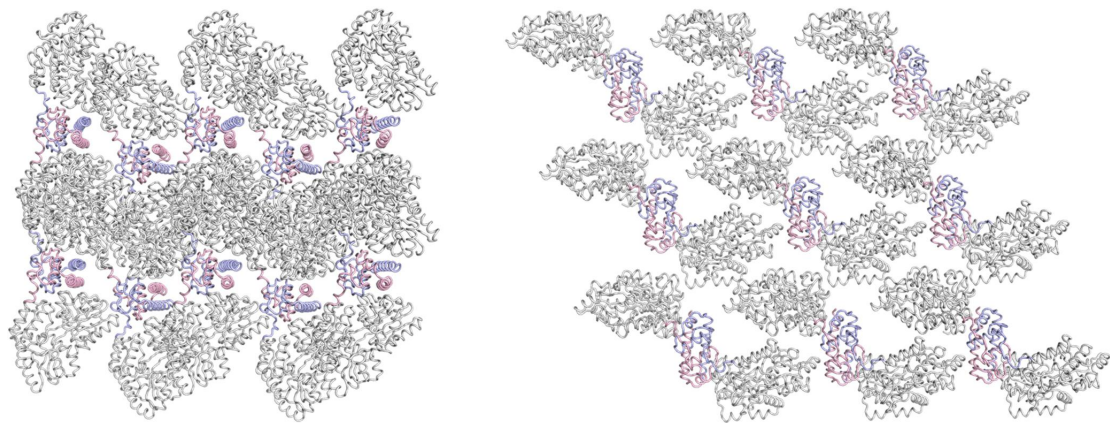
Supplementary information, Figure S3. The packing mode of ZIKVCC in the high-resolution crystals. The two ZIKV C protomers are colored in light blue and light pink, respectively; MBP is in gray.
