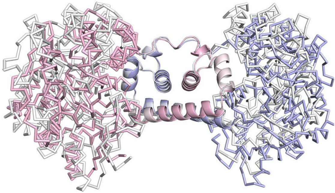
Supplementary information, Figure S4. The structural alignment of ZIKV C proteins in the two different crystals. The crystal structure at a high-resolution colored in light blue and light pink; the low-resolution structure was colored in gray.
