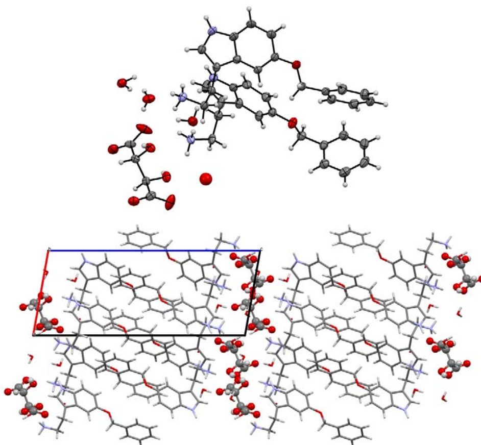
Supplementary Figure 8: Top: displacement ellipsoid representation of [\text{BaH}]_2[\text{L-tartrate}] \cdot 3.35(\text{H}_2\text{O}) , ellipsoids are drawn at 50% probability. Only the major conformer of the disordered ethylammonium group is shown for clarity. Below: packing diagram of [\text{BaH}]_2[\text{L-tartrate}] \cdot 3.35(\text{H}_2\text{O}) .
