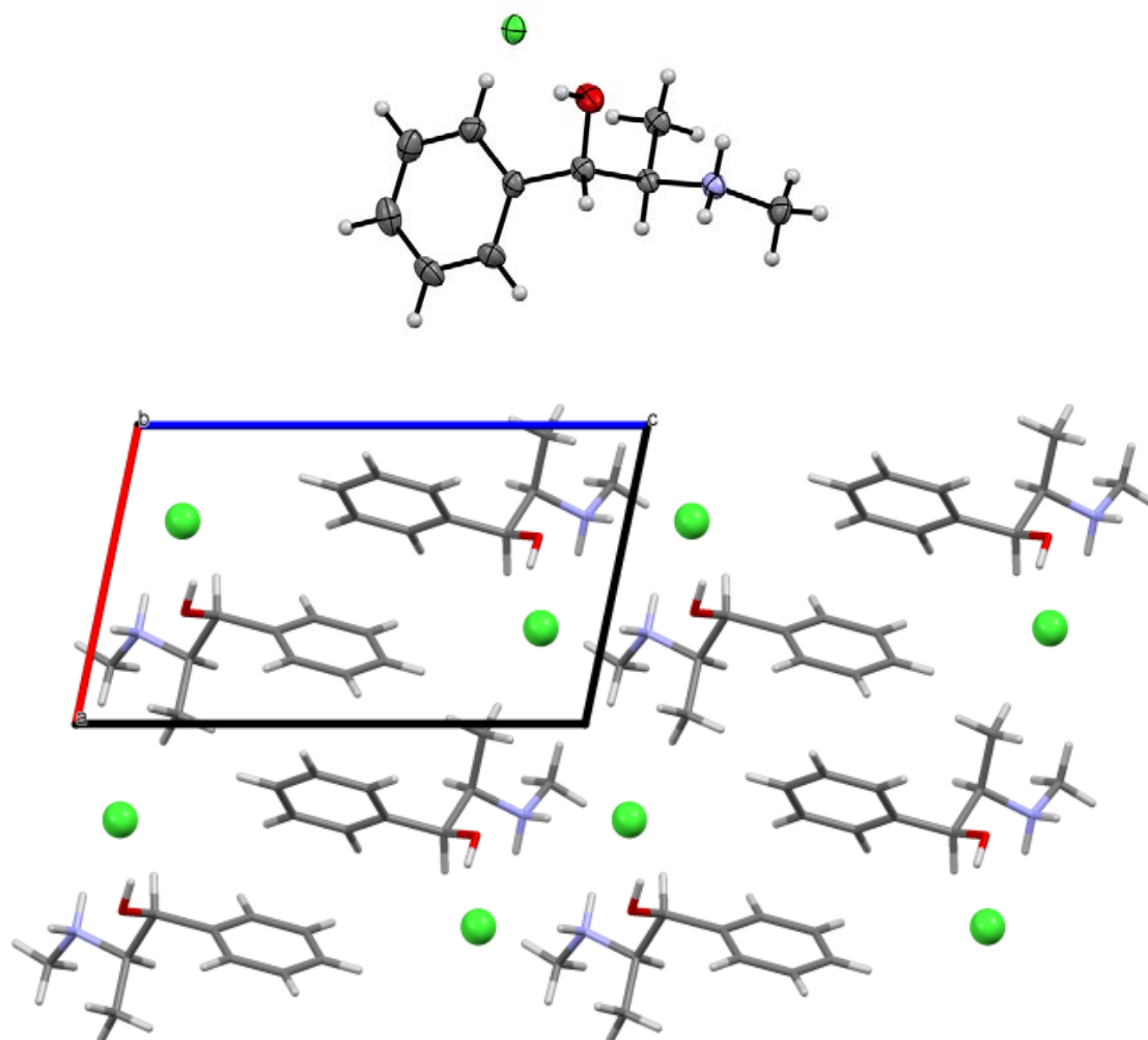
Supplementary Figure 17: Top: displacement ellipsoid representation of [(1 S ,2 R )-(+)-ephedrinium][chloride] , ellipsoids are drawn at 50% probability. Below: packing diagram of [(1 S ,2 R )-(+)-ephedrinium][chloride] .
