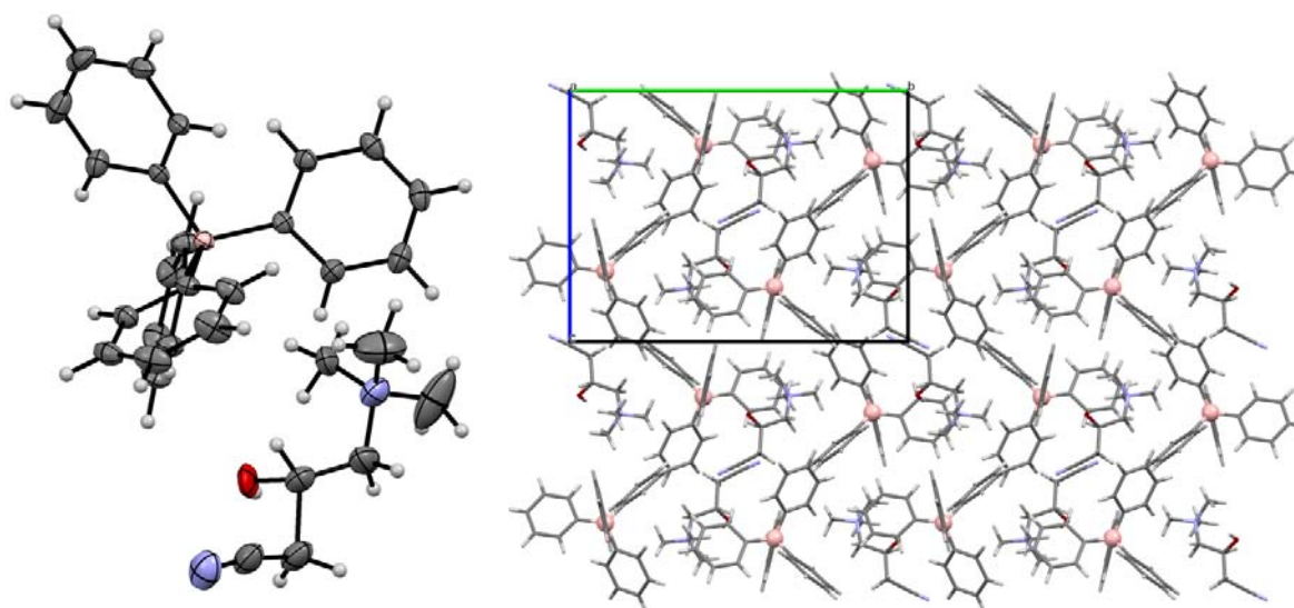
Supplementary Figure 13: Left: displacement ellipsoid representation of [( R,S )-carnitinenitrile][tetraphenylborate], ellipsoids are drawn at 50% probability. Only the major conformer of the disordered hydroxy part is shown for clarity. Right: packing diagram of [( R,S )-carnitinenitrile][tetraphenylborate].
