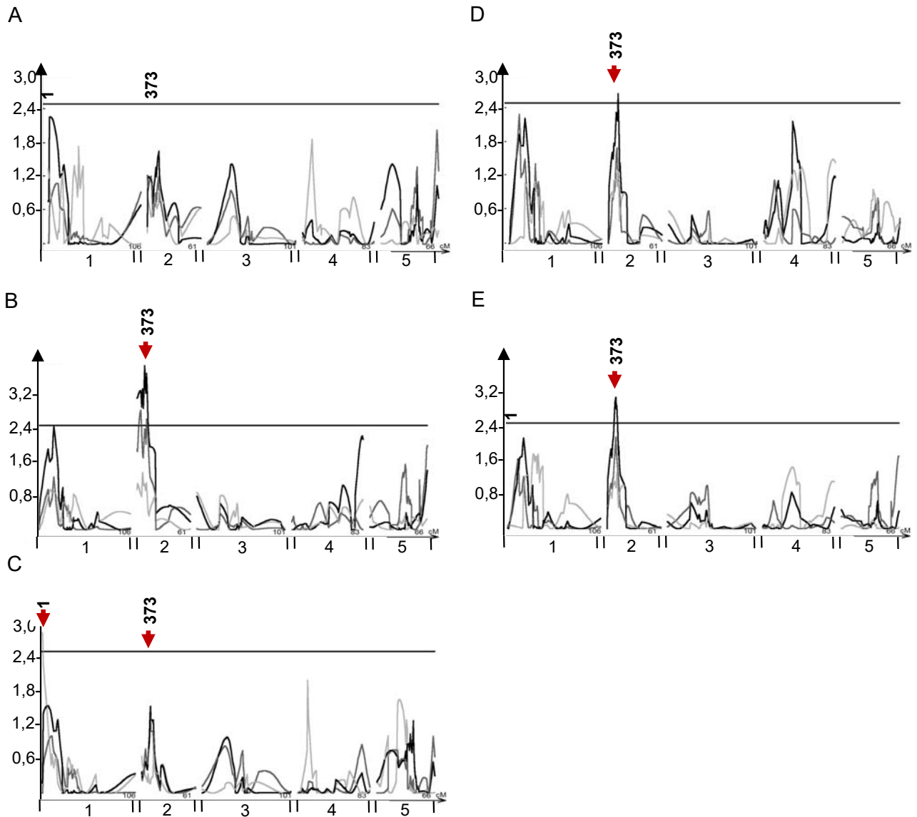
Figure S1: EpiQTL mapping of LC glucosinolate means. Plots show composite interval mapping results and significance estimated from 1000 permutations. The x-axis shows the genome by chromosome and y-axis shows the LOD score. The significance thresholds are plotted for each trait and significant QTLs are re marked with red arrows. The light grey line shows the QTL map using the means from experiment 1, dark grey shows experiment 2, and black lines represent the pooled data from experiment 1 and 2. Marker names show the position of significant makers after using a linear model to assess loci. An asterisk after a marker shows that the marker was not significant in both experiments. EpiQTLs not assigned a marker were rejected in the subsequent ANOVA. Analyzed LC glucosinolates are A) 7MTH, B) 7MSH, C) 8MTO, D) 8MSO, E) Pooled LC glucosinolates.
