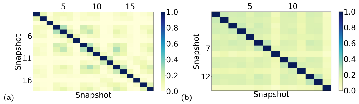
Fig S1. Pairwise edge overlaps between the snapshots of social (a) hospital and (b) high school dynamic networks. The darker the color, the higher the edge overlap between the given snapshots. For the hospital data, the following network construction parameter values are used: t_w=300 seconds and w=1 . For the high school data, the parameter values are: t_w=200 seconds and w=1 .
