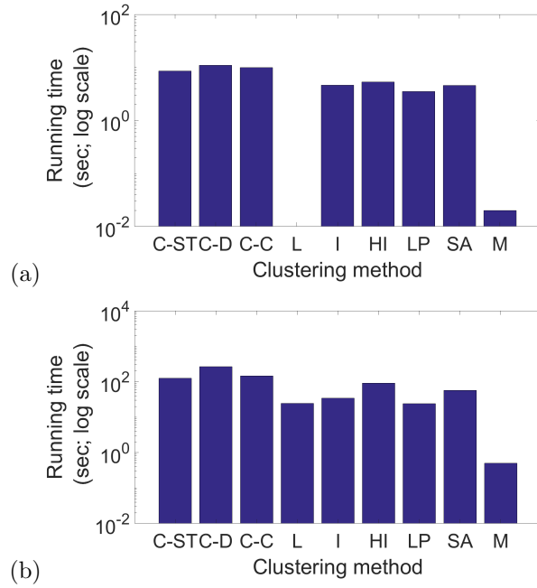
Fig S8. Running time comparison. Running time comparison of the different methods (ClueNet (its three versions: C-ST, C-D, C-C), Louvain (L), Infomap (I), Hierarchical Infomap (HI), label propagation (LP), simulated annealing (SA), and Multistep (M)) for the social (a) hospital and (b) high school dynamic networks.
