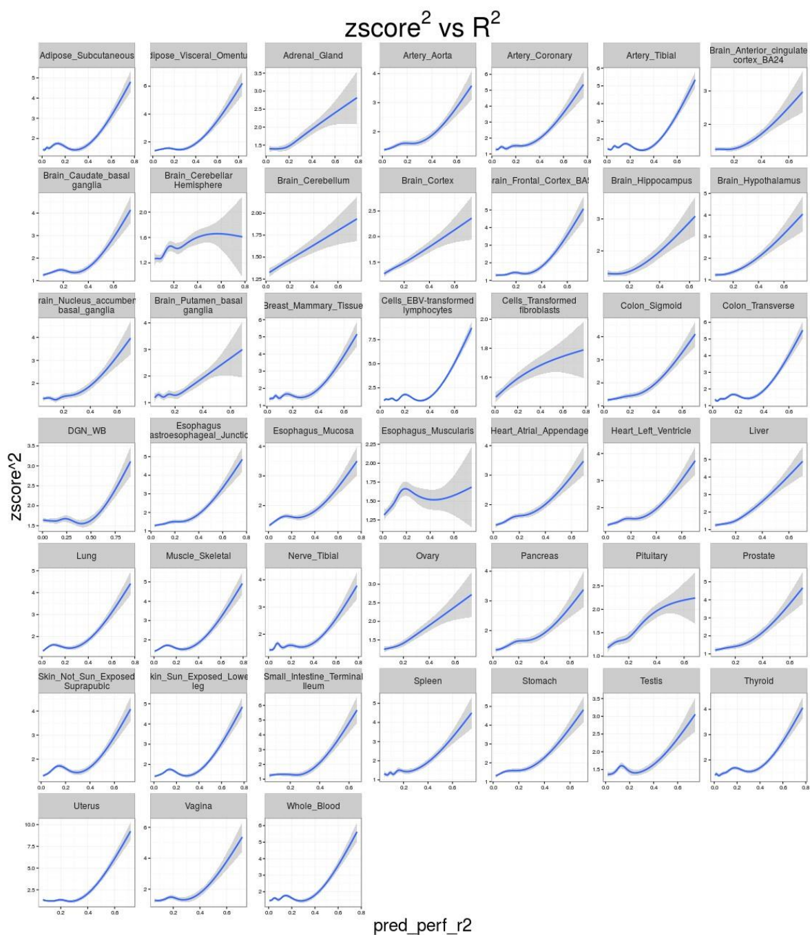
Supplementary Figure 2: Z-score 2 vs predicted performance R 2 by tissue
