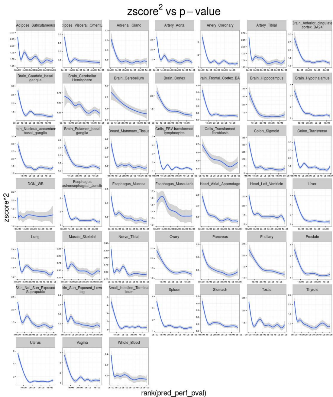
Supplementary Figure 4: Z-score 2 vs predicted performance p-value by tissue
