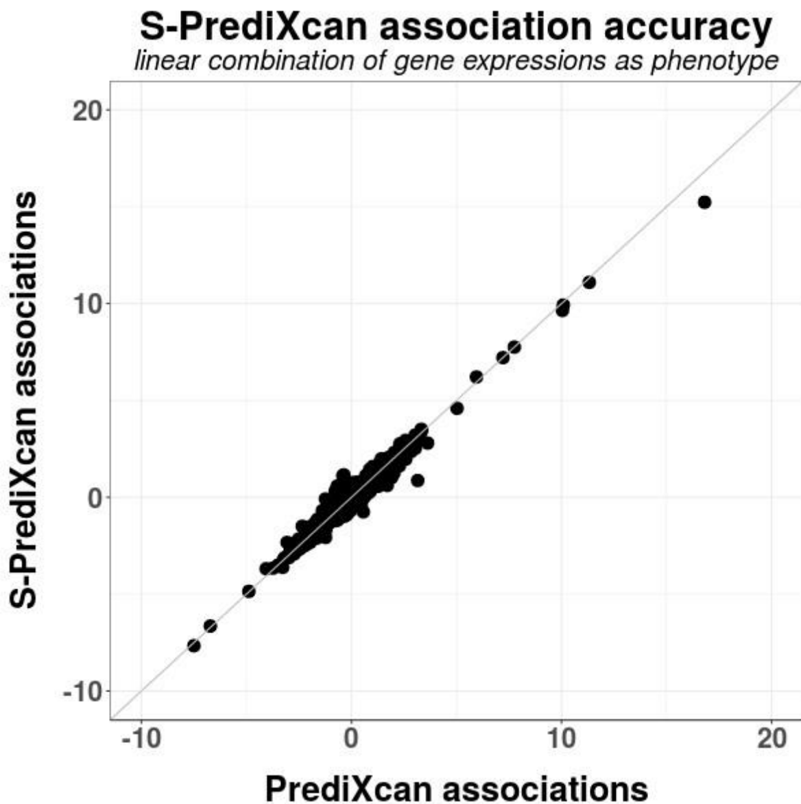
Supplementary Figure 11: S-PrediXcan Associations for a simulated phenotype under the alternative hypothesis
